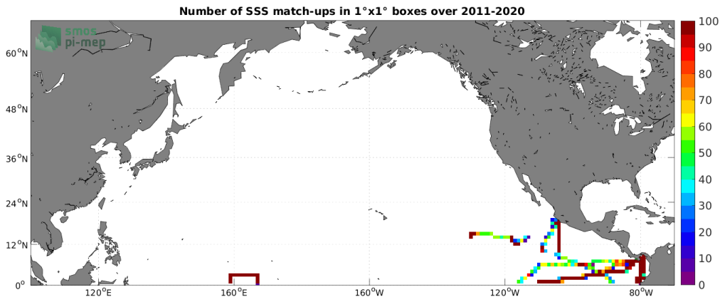
Figure 4: Number of SSS match-ups between TSG (GOSUD-Research-vessel) SSS and the SMOS SSS L4 OI v342 - Weekly (CMEMS-CATDS-LOPS) SSS product for the North Pacific Ocean Pi-MEP region over 1^\circ \times 1^\circ boxes and for the full satellite product period.
