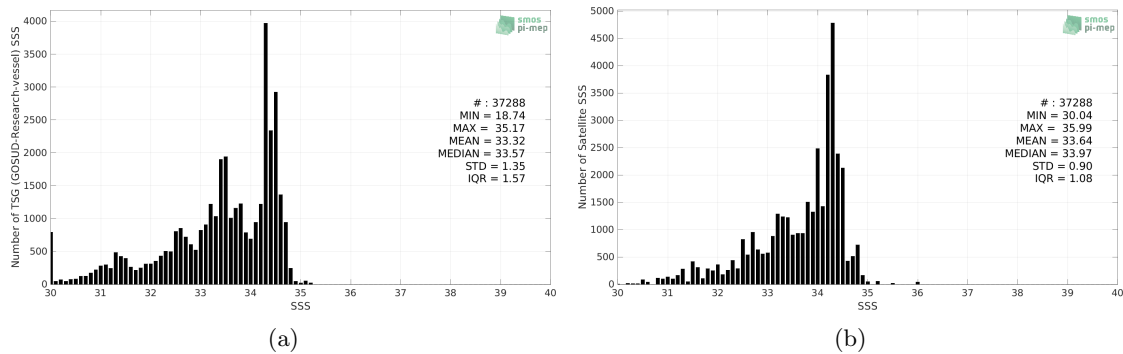
Figure 2: Histograms of SSS from TSG (GOSUD-Research-vessel) (a) and SMOS SSS L4 OI v342 - Weekly (CMEMS-CATDS-LOPS) (b) considering all match-up pairs per bins of 0.1 over the North Pacific Ocean Pi-MEP region and for the full satellite product period.
