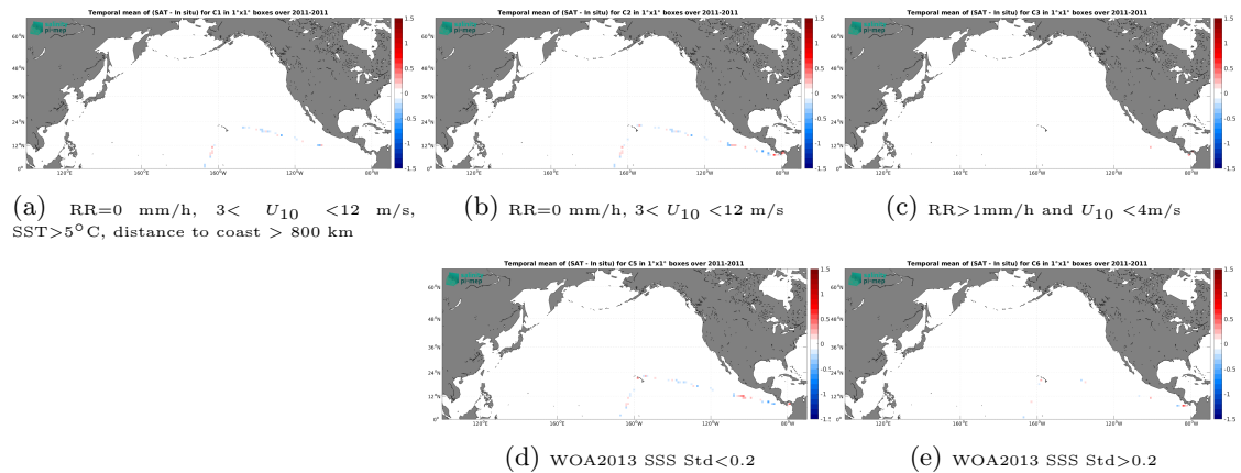
Figure 12: Temporal mean gridded over spatial boxes of size 1^\circ \times 1^\circ of \Delta SSS (SMOS SSS L4 OI v342 - Weekly (CMEMS-CATDS-LOPS) - TSG (CSIC-UTM)) for 5 different subdatasets corresponding to:RR=0 mm/h, 3 < U_{10} < 12 m/s, SST >5^\circ C, distance to coast > 800 km (a), RR=0 mm/h, 3 < U_{10} < 12 m/s (b), RR >1 mm/h and U_{10} < 4 m/s (c), WOA2013 SSS Std <0.2 (d), WOA2013 SSS Std >0.2 (e).
