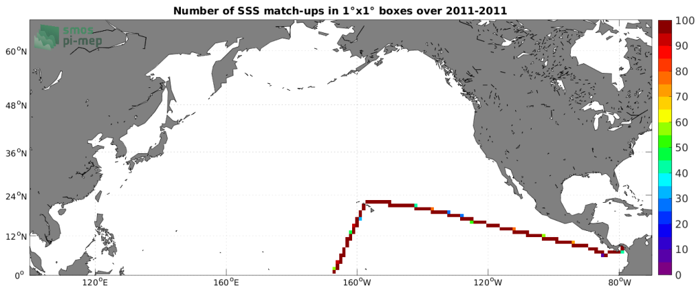
Figure 4: Number of SSS match-ups between TSG (CSIC-UTM) SSS and the SMOS SSS L4 OI v342 - Weekly (CMEMS-CATDS-LOPS) SSS product for the North Pacific Ocean Pi-MEP region over 1^\circ \times 1^\circ boxes and for the full satellite product period.
