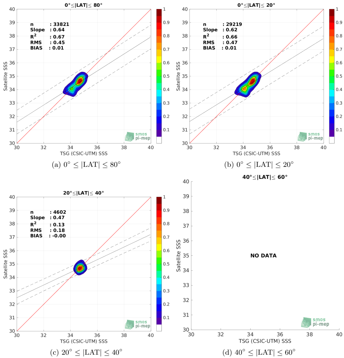
Figure 9: Contour maps of the concentration of SMOS SSS L4 OI v342 - Weekly (CMEMS-CATDS-LOPS) SSS (y-axis) versus TSG (CSIC-UTM) SSS (x-axis) at match-up pairs for different latitude bands. For each plot, the red line shows x=y . The black thin and dashed lines indicate a linear fit through the data cloud and the \pm 95\% confidence levels, respectively. The number match-up pairs n , the slope and R^2 coefficient of the linear fit, the root mean square (RMS) and the mean bias between satellite and in situ data are indicated for each latitude band in each plots.
