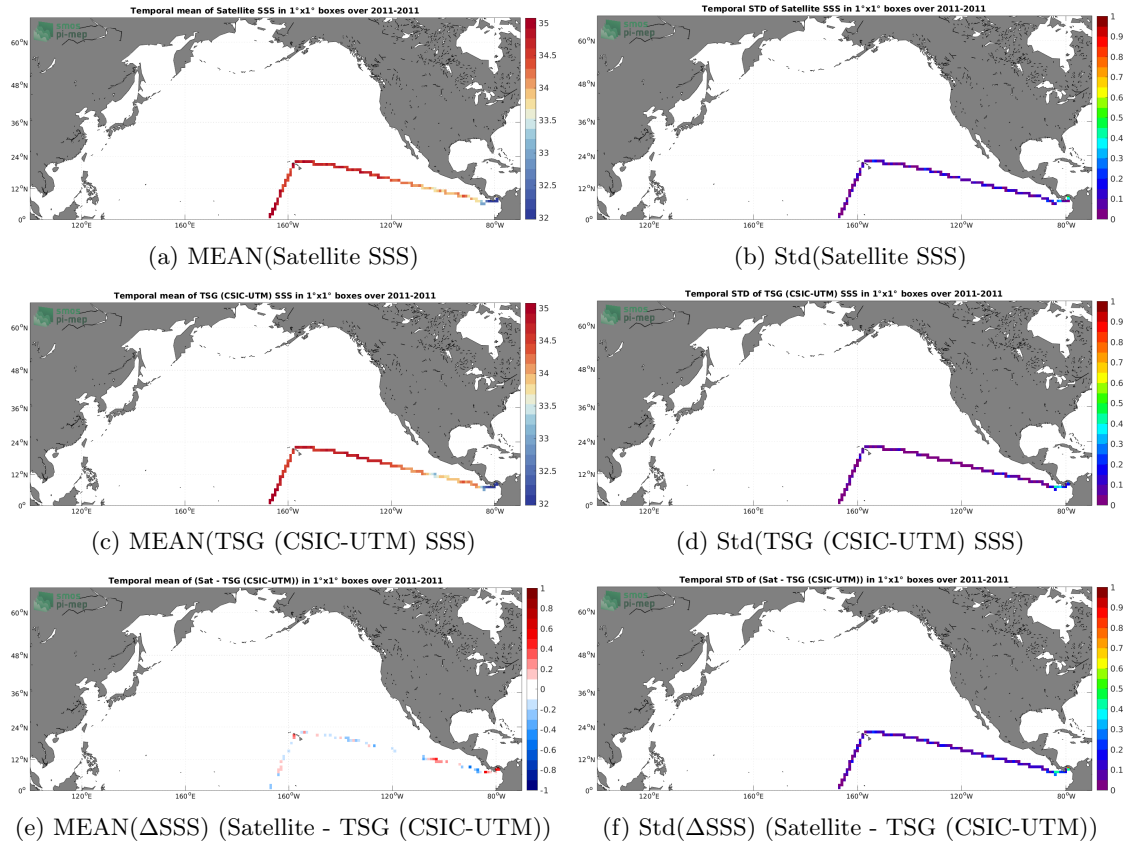
Figure 6: Temporal mean (left) and Std (right) of SSS from SMOS SSS L4 OI v342 - Weekly (CMEMS-CATDS-LOPS) (top), TSG (CSIC-UTM) (middle), and of \Delta SSS (Satellite - TSG (CSIC-UTM)). Only match-up pairs are used to generate these maps.
