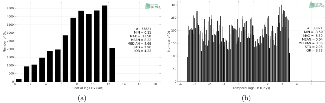
Figure 5: Histograms of the spatial (a) and temporal (b) lags between the location/time of the TSG (CSIC-UTM) measurement and the date of the corresponding SMOS SSS L4 OI v342 - Weekly (CMEMS-CATDS-LOPS) SSS pixel.
