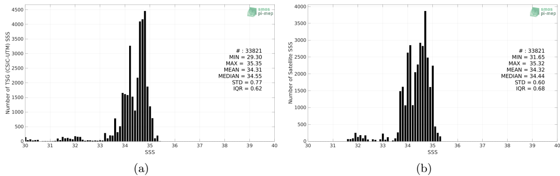
Figure 2: Histograms of SSS from TSG (CSIC-UTM) (a) and SMOS SSS L4 OI v342 - Weekly (CMEMS-CATDS-LOPS) (b) considering all match-up pairs per bins of 0.1 over the North Pacific Ocean Pi-MEP region and for the full satellite product period.
