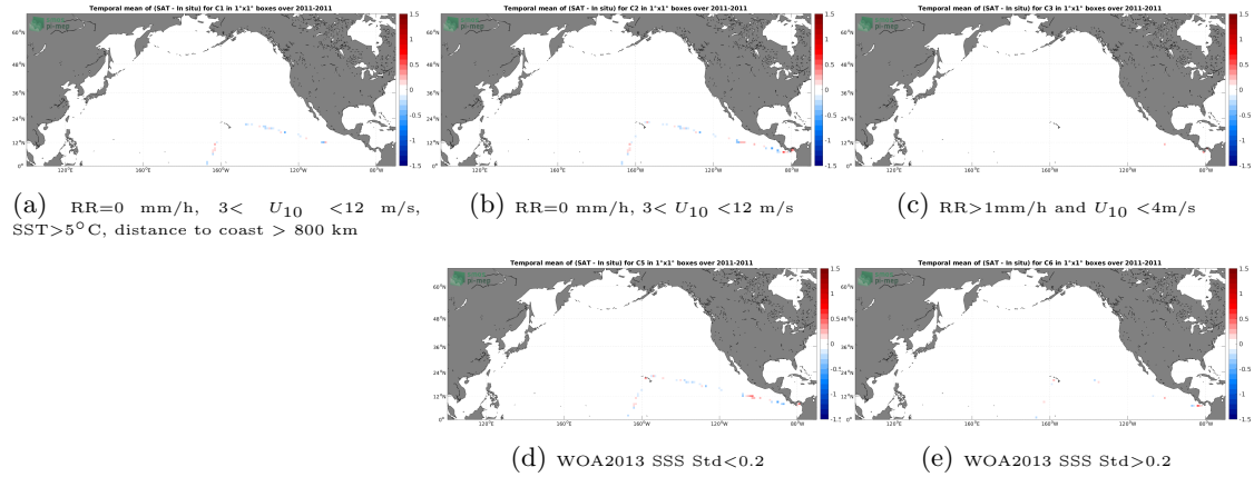
Figure 12: Temporal mean gridded over spatial boxes of size 1^{\circ}\times 1^{\circ} of \Delta\text{SSS} (SMOS SSS L4 OI v342 - Weekly (CMEMS-CATDS-LOPS) - TSG (CSIC-UTM)) for 5 different subdatasets corresponding to:RR=0 mm/h, 3 < U_{10} < 12 m/s, SST >5^{\circ}\text{C} , distance to coast > 800 km (a), RR=0 mm/h, 3 < U_{10} < 12 m/s (b), RR >1 mm/h and U_{10} < 4 m/s (c), WOA2013 SSS Std <0.2 (d), WOA2013 SSS Std >0.2 (e).
