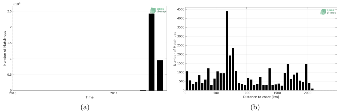
Figure 1: Number of match-ups between TSG (CSIC-UTM) and SMOS SSS L4 OI v342 - Weekly (CMEMS-CATDS-LOPS) SSS as a function of time (a) and as function of the distance to coast (b) over the North Pacific Ocean Pi-MEP region and for the full satellite product period.
