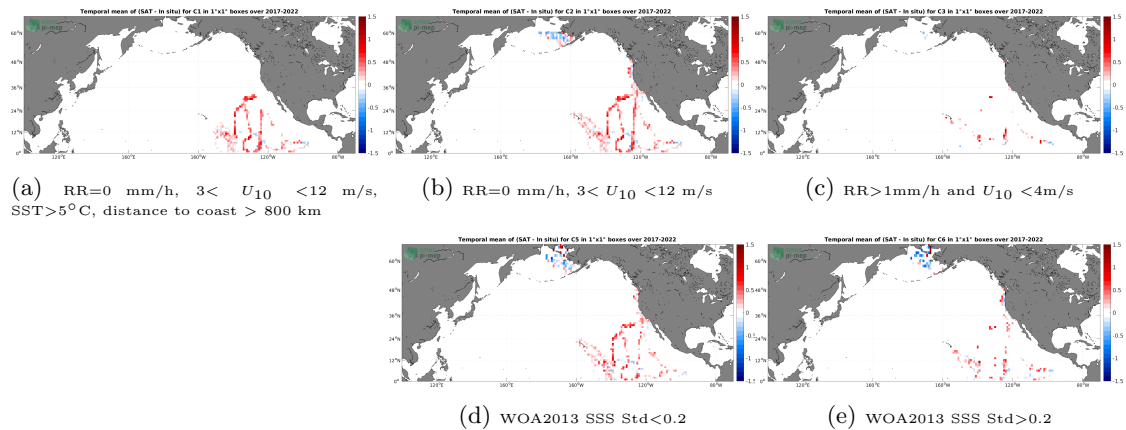
Figure 12: Temporal mean gridded over spatial boxes of size 1^\circ \times 1^\circ of \Delta SSS (SMOS SSS L4 OI v342 - Weekly (CMEMS-CATDS-LOPS) - Sailydrone) for 5 different subdatasets corresponding to:RR=0 mm/h, 3 < U_{10} < 12 m/s, SST >5^\circ C, distance to coast > 800 km (a), RR=0 mm/h, 3 < U_{10} < 12 m/s (b), RR >1 mm/h and U_{10} < 4 m/s (c), WOA2013 SSS Std <0.2 (d), WOA2013 SSS Std >0.2 (e).
