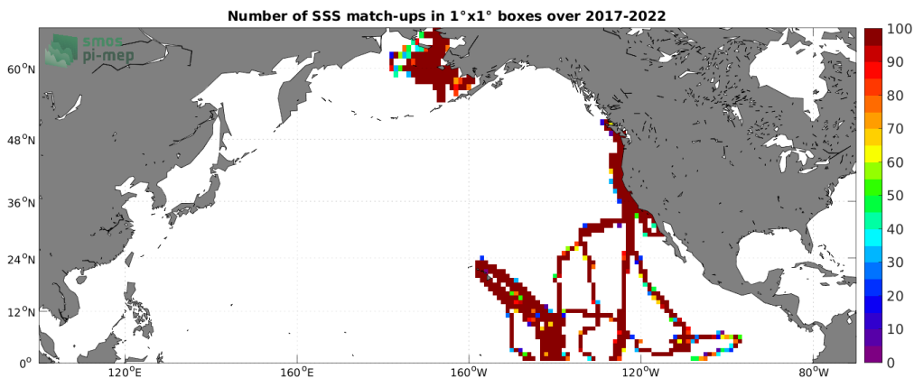
Figure 4: Number of SSS match-ups between Saildrone SSS and the SMOS SSS L4 OI v342 - Weekly (CMEMS-CATDS-LOPS) SSS product for the North Pacific Ocean Pi-MEP region over 1^\circ \times 1^\circ boxes and for the full satellite product period.
