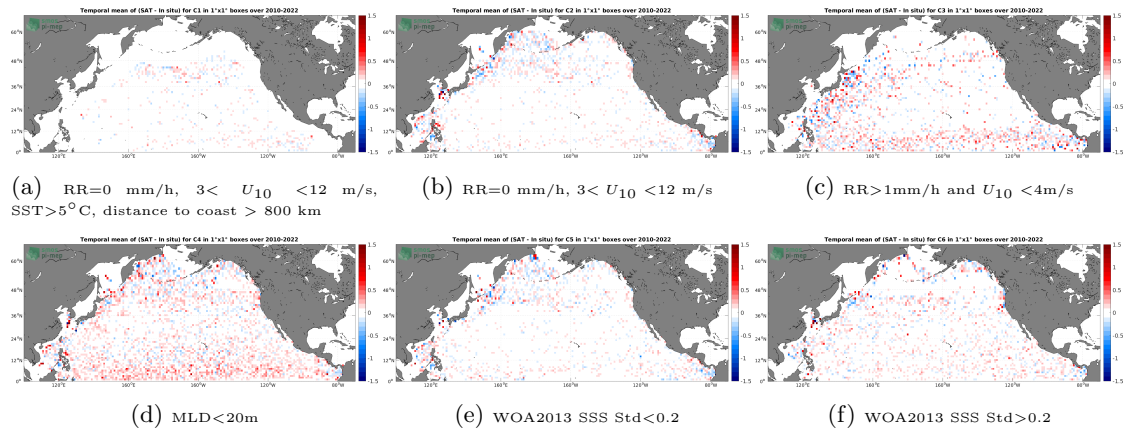
Figure 12: Temporal mean gridded over spatial boxes of size 1^\circ \times 1^\circ of \Delta SSS (SMOS SSS L4 OI v342 - Weekly (CMEMS-CATDS-LOPS) - Argo) for 6 different subdatasets corresponding to:RR=0 mm/h, 3 < U_{10} < 12 m/s, SST >5^\circ C, distance to coast > 800 km (a), RR=0 mm/h, 3 < U_{10} < 12 m/s (b), RR >1 mm/h and U_{10} < 4 m/s (c),MLD <20 m (d),WOA2013 SSS Std <0.2 (e),WOA2013 SSS Std >0.2 (f).
