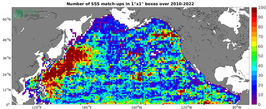
Figure 4: Number of SSS match-ups between Argo SSS and the SMOS SSS L4 OI v342 - Weekly (CMEMS-CATDS-LOPS) SSS product for the North Pacific Ocean Pi-MEP region over 1^\circ \times 1^\circ boxes and for the full satellite product period.
