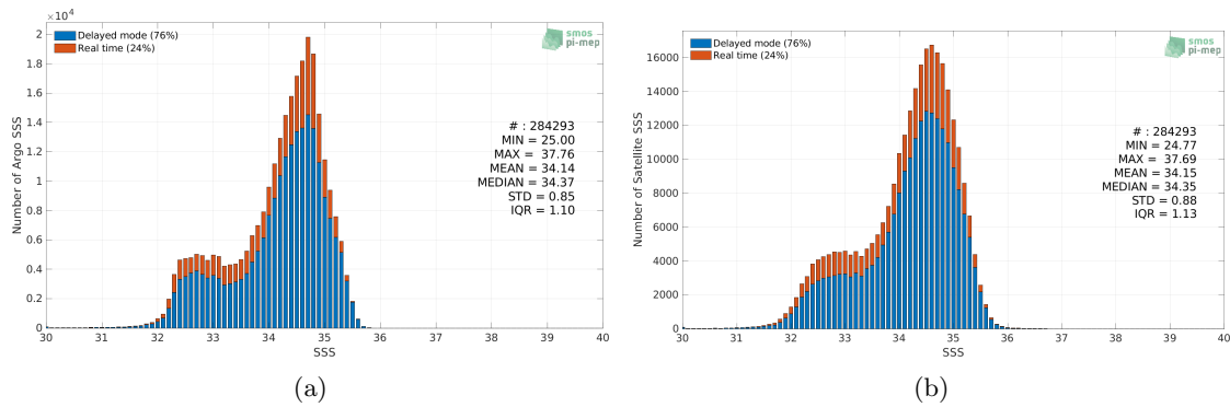
Figure 2: Histograms of SSS from Argo (a) and SMOS SSS L4 OI v342 - Weekly (CMEMS-CATDS-LOPS) (b) considering all match-up pairs per bins of 0.1 over the North Pacific Ocean Pi-MEP region and for the full satellite product period.
