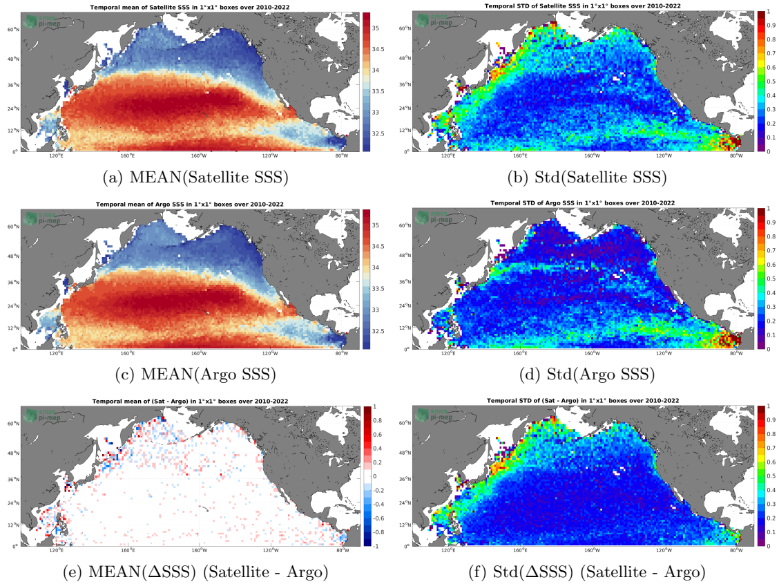
Figure 6: Temporal mean (left) and Std (right) of SSS from SMOS SSS L4 OI v342 - Weekly (CMEMS-CATDS-LOPS) (top), Argo (middle), and of \Delta SSS (Satellite - Argo). Only match-up pairs are used to generate these maps.
