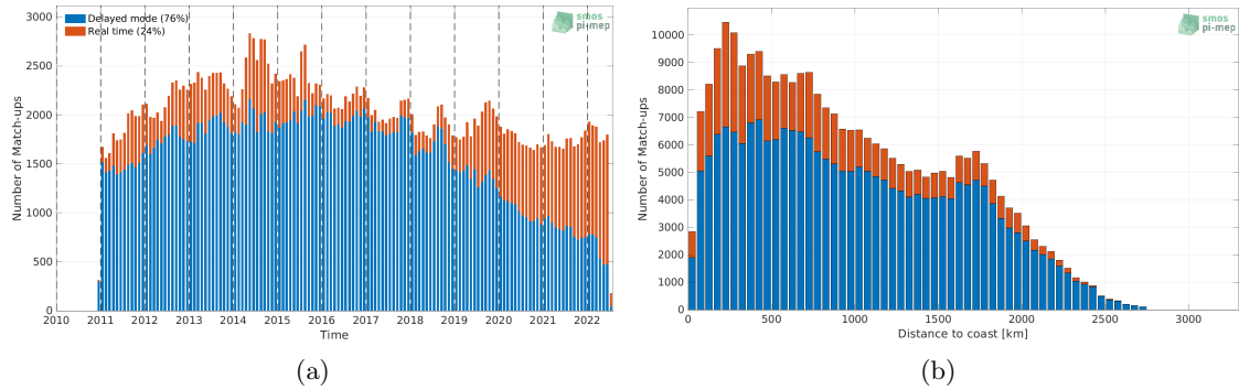
Figure 1: Number of match-ups between Argo and SMOS SSS L4 OI v342 - Weekly (CMEMS-CATDS-LOPS) SSS as a function of time (a) and as function of the distance to coast (b) over the North Pacific Ocean Pi-MEP region and for the full satellite product period.
