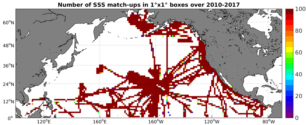
Figure 4: Number of SSS match-ups between TSG-SAMOS SSS and the SMOS-L4-CATDS-CECOS-IFREMER-V2-WEEKLY-0.5DEG SSS product for the North Pacific Ocean Pi-MEP region over 1°x1° boxes and for the full satellite product period.
