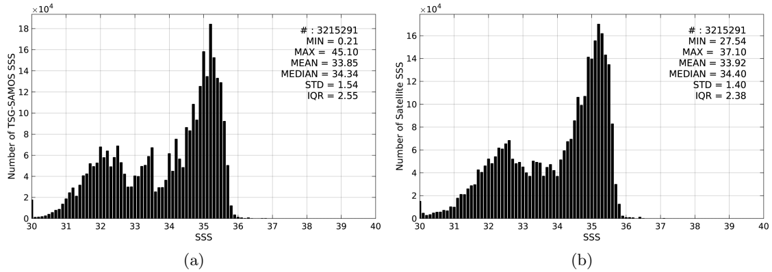
Figure 2: Histograms of SSS from TSG-SAMOS (a) and SMOS-L4-CATDS-CECOS-IFREMER-V2-WEEKLY-0.5DEG (b) considering all match-up pairs per bins of 0.1 over the North Pacific Ocean Pi-MEP region and for the full satellite product period.
