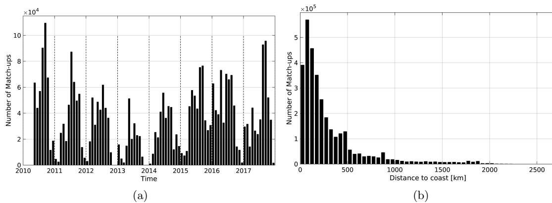
Figure 1: Number of match-ups between TSG-SAMOS and SMOS-L4-CATDS-CECOS-IFREMER-V2-WEEKLY-0.5DEG SSS as a function of time (a) and as function of the distance to coast (b) over the North Pacific Ocean Pi-MEP region and for the full satellite product period.
