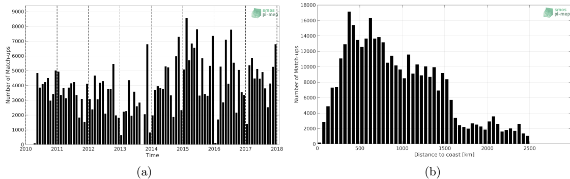
Figure 1: Number of match-ups between TSG (LEGOS-DM) and SMOS L4 v2 Weekly (CATDS-CECOS-IFREMER) SSS as a function of time (a) and as function of the distance to coast (b) over the North Pacific Ocean Pi-MEP region and for the full satellite product period.
