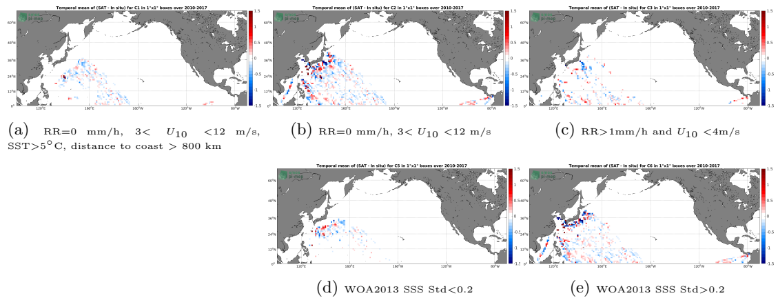
Figure 12: Temporal mean gridded over spatial boxes of size 1^\circ \times 1^\circ of \Delta SSS (SMOS L4 v2 Weekly (CATDS-CECOS-IFREMER) - TSG (LEGOS-DM)) for 5 different subdatasets corresponding to:RR=0 mm/h, 3 < U_{10} < 12 m/s, SST>5°C, distance to coast > 800 km (a), RR=0 mm/h, 3 < U_{10} < 12 m/s (b), RR>1mm/h and U_{10} < 4 m/s (c), WOA2013 SSS Std<0.2 (d), WOA2013 SSS Std>0.2 (e).
