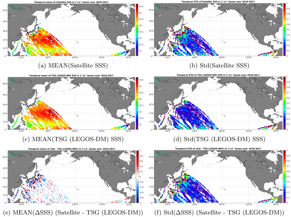
Figure 6: Temporal mean (left) and Std (right) of SSS from SMOS L4 v2 Weekly (CATDS-CECOS-IFREMER) (top), TSG (LEGOS-DM) (middle), and of \Delta\text{SSS} (Satellite - TSG (LEGOS-DM)). Only match-up pairs are used to generate these maps.
