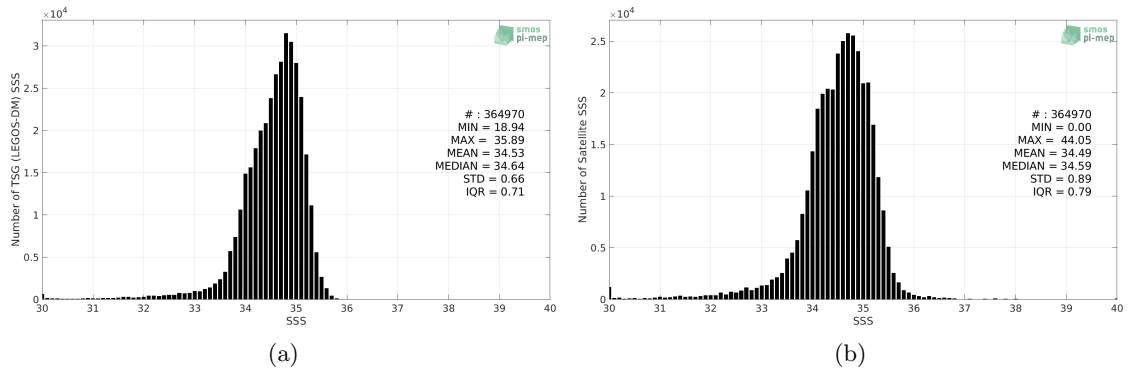
Figure 2: Histograms of SSS from TSG (LEGOS-DM) (a) and SMOS L4 v2 Weekly (CATDS-CECOS-IFREMER) (b) considering all match-up pairs per bins of 0.1 over the North Pacific Ocean Pi-MEP region and for the full satellite product period.
