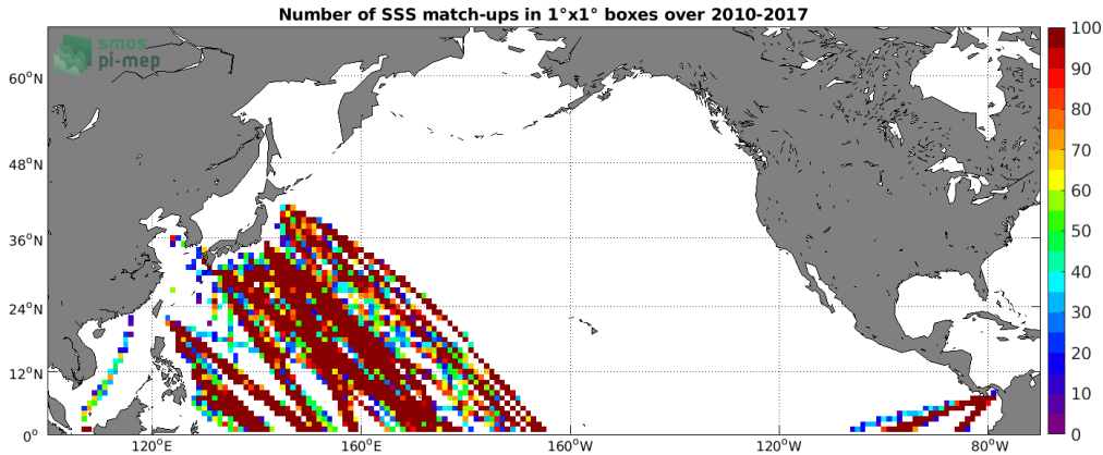
Figure 4: Number of SSS match-ups between TSG (LEGOS-DM) SSS and the SMOS L4 v2 Weekly (CATDS-CECOS-IFREMER) SSS product for the North Pacific Ocean Pi-MEP region over 1^\circ \times 1^\circ boxes and for the full satellite product period.
