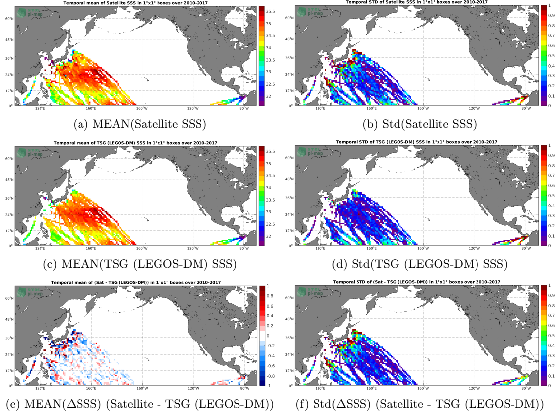
Figure 6: Temporal mean (left) and Std (right) of SSS from SMOS L4 v2 Weekly (CATDS-CECOS-IFREMER) (top), TSG (LEGOS-DM) (middle), and of \Delta SSS (Satellite - TSG (LEGOS-DM)). Only match-up pairs are used to generate these maps.
