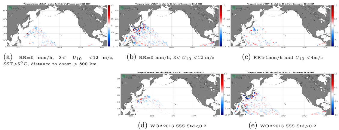
Figure 12: Temporal mean gridded over spatial boxes of size 1°x1° of \Delta SSS (SMOS L4 v2 Weekly (CATDS-CECOS-IFREMER) - TSG (LEGOS-DM)) for 5 different subdatasets corresponding to:RR=0 mm/h, 3 < U_{10} < 12 m/s, SST>5°C, distance to coast > 800 km (a), RR=0 mm/h, 3 < U_{10} < 12 m/s (b), RR>1mm/h and U_{10} < 4 m/s (c), WOA2013 SSS Std<0.2 (d), WOA2013 SSS Std>0.2 (e).
