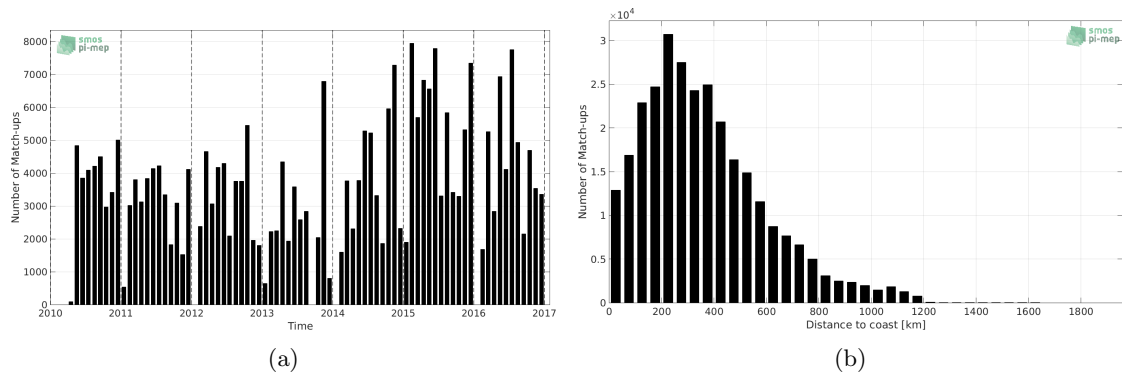
Figure 1: Number of match-ups between TSG-LEGOS-DM and SMOS-L4-CATDS-CECOS-IFREMER-V2-WEEKLY-0.5DEG SSS as a function of time (a) and as function of the distance to coast (b) over the North Pacific Ocean Pi-MEP region and for the full satellite product period.
