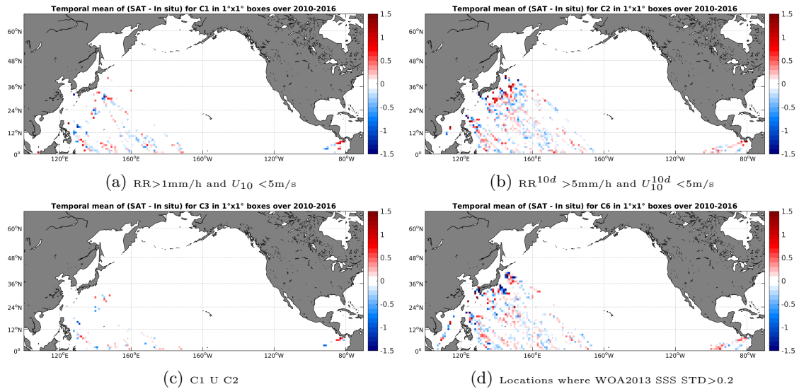
Figure 12: Temporal mean gridded over spatial boxes of size 1^\circ \times 1^\circ of \Delta SSS (SMOS-L4-CATDS-CECOS-IFREMER-V2-WEEKLY-0.5DEG - TSG-LEGOS-DM) for 4 different subdatasets corresponding to: RR > 1\text{mm/h} and U_{10} < 5\text{m/s} (a), RR^{10d} > 5\text{mm/h} and U_{10}^{10d} < 5\text{m/s} (b), C1 U C2 (c), Locations where WOA2013 SSS STD > 0.2 (d).
