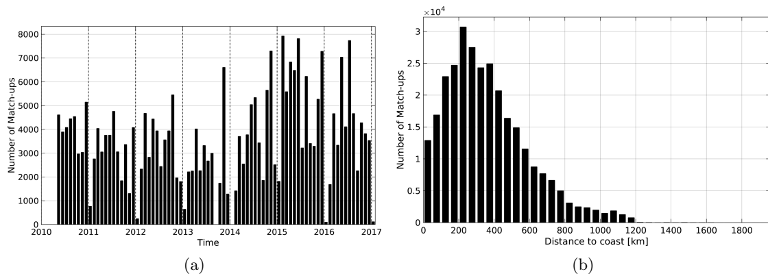
Figure 1: Number of match-ups between TSG-LEGOS-DM and SMOS-L4-CATDS-CECOS-IFREMER-V2-WEEKLY-0.5DEG SSS as a function of time (a) and as function of the distance to coast (b) over the North Pacific Ocean Pi-MEP region and for the full satellite product period.
