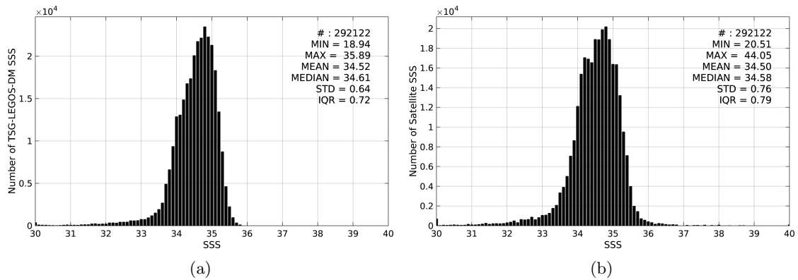
Figure 2: Histograms of SSS from TSG-LEGOS-DM (a) and SMOS-L4-CATDS-CECOS-IFREMER-V2-WEEKLY-0.5DEG (b) considering all match-up pairs per bins of 0.1 over the North Pacific Ocean Pi-MEP region and for the full satellite product period.
