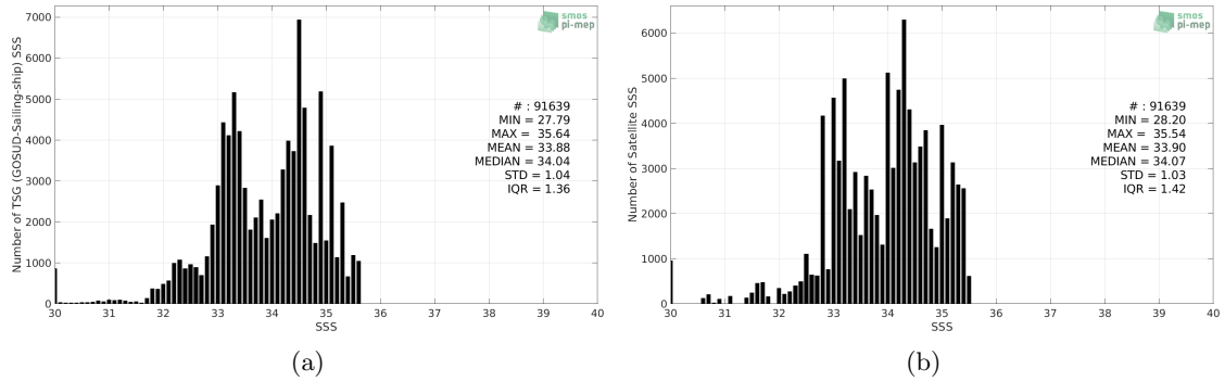
Figure 2: Histograms of SSS from TSG (GOSUD-Sailing-ship) (a) and SMOS L4 v2 Weekly (CATDS-CECOS-IFREMER) (b) considering all match-up pairs per bins of 0.1 over the North Pacific Ocean Pi-MEP region and for the full satellite product period.
