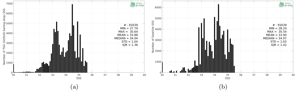
Figure 2: Histograms of SSS from TSG (GOSUD-Sailing-ship) (a) and SMOS L4 v2 Weekly (CATDS-CECOS-IFREMER) (b) considering all match-up pairs per bins of 0.1 over the North Pacific Ocean Pi-MEP region and for the full satellite product period.
