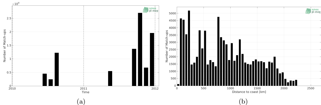
Figure 1: Number of match-ups between TSG (GOSUD-Sailing-ship) and SMOS L4 v2 Weekly (CATDS-CECOS-IFREMER) SSS as a function of time (a) and as function of the distance to coast (b) over the North Pacific Ocean Pi-MEP region and for the full satellite product period.
