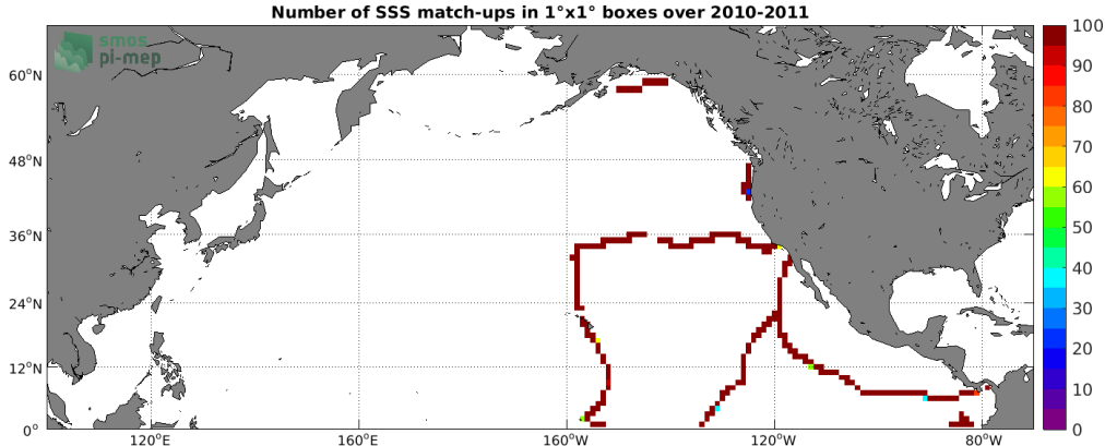
Figure 4: Number of SSS match-ups between TSG (GOSUD-Sailing-ship) SSS and the SMOS L4 v2 Weekly (CATDS-CECOS-IFREMER) SSS product for the North Pacific Ocean Pi-MEP region over 1^\circ \times 1^\circ boxes and for the full satellite product period.
