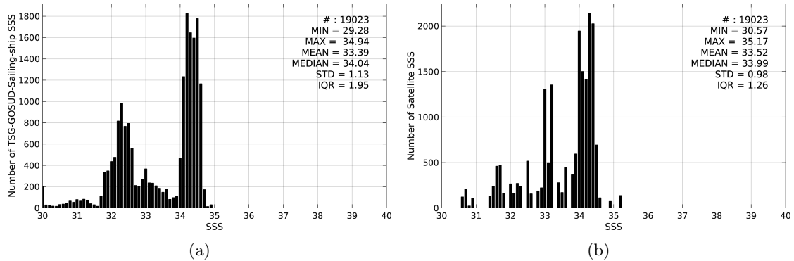
Figure 2: Histograms of SSS from TSG-GOSUD-Sailing-ship (a) and SMOS-L4-CATDS-CECOS-IFREMER-V2-WEEKLY-0.5DEG (b) considering all match-up pairs per bins of 0.1 over the North Pacific Ocean Pi-MEP region and for the full satellite product period.
