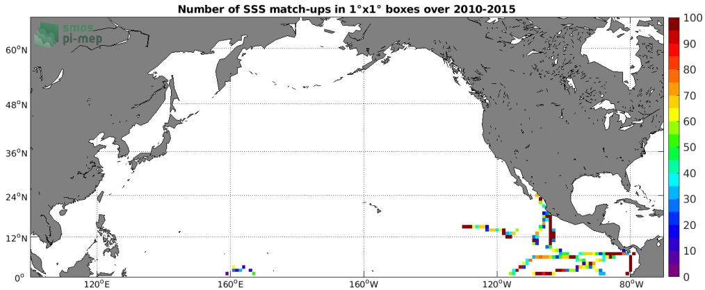
Figure 4: Number of SSS match-ups between TSG (GOSUD-Research-vessel) SSS and the SMOS L4 v2 Weekly (CATDS-CECOS-IFREMER) SSS product for the North Pacific Ocean Pi-MEP region over 1^\circ \times 1^\circ boxes and for the full satellite product period.
