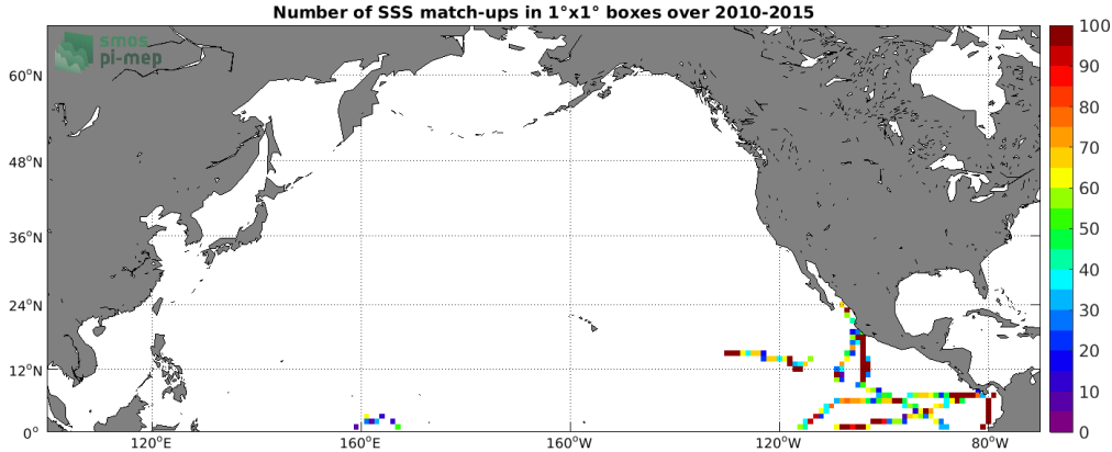
Figure 4: Number of SSS match-ups between TSG (GOSUD-Research-vessel) SSS and the SMOS L4 v2 Weekly (CATDS-CECOS-IFREMER) SSS product for the North Pacific Ocean Pi-MEP region over 1°x1° boxes and for the full satellite product period.
