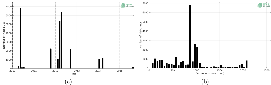
Figure 1: Number of match-ups between TSG (GOSUD-Research-vessel) and SMOS L4 v2 Weekly (CATDS-CECOS-IFREMER) SSS as a function of time (a) and as function of the distance to coast (b) over the North Pacific Ocean Pi-MEP region and for the full satellite product period.
