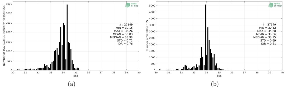
Figure 2: Histograms of SSS from TSG (GOSUD-Research-vessel) (a) and SMOS L4 v2 Weekly (CATDS-CECOS-IFREMER) (b) considering all match-up pairs per bins of 0.1 over the North Pacific Ocean Pi-MEP region and for the full satellite product period.
