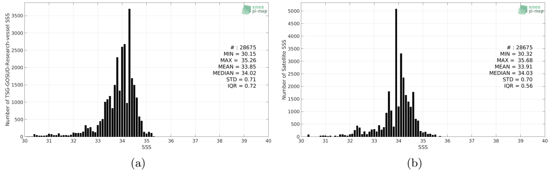
Figure 2: Histograms of SSS from TSG-GOSUD-Research-vessel (a) and SMOS-L4-CATDS-CECOS-IFREMER-V2-WEEKLY-0.5DEG (b) considering all match-up pairs per bins of 0.1 over the North Pacific Ocean Pi-MEP region and for the full satellite product period.
