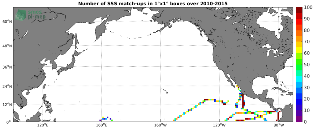
Figure 4: Number of SSS match-ups between TSG-GOSUD-Research-vessel SSS and the SMOS-L4-CATDS-CECOS-IFREMER-V2-WEEKLY-0.5DEG SSS product for the North Pacific Ocean Pi-MEP region over 1^\circ \times 1^\circ boxes and for the full satellite product period.
