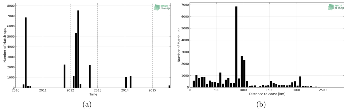
Figure 1: Number of match-ups between TSG-GOSUD-Research-vessel and SMOS-L4-CATDS-CECOS-IFREMER-V2-WEEKLY-0.5DEG SSS as a function of time (a) and as function of the distance to coast (b) over the North Pacific Ocean Pi-MEP region and for the full satellite product period.
