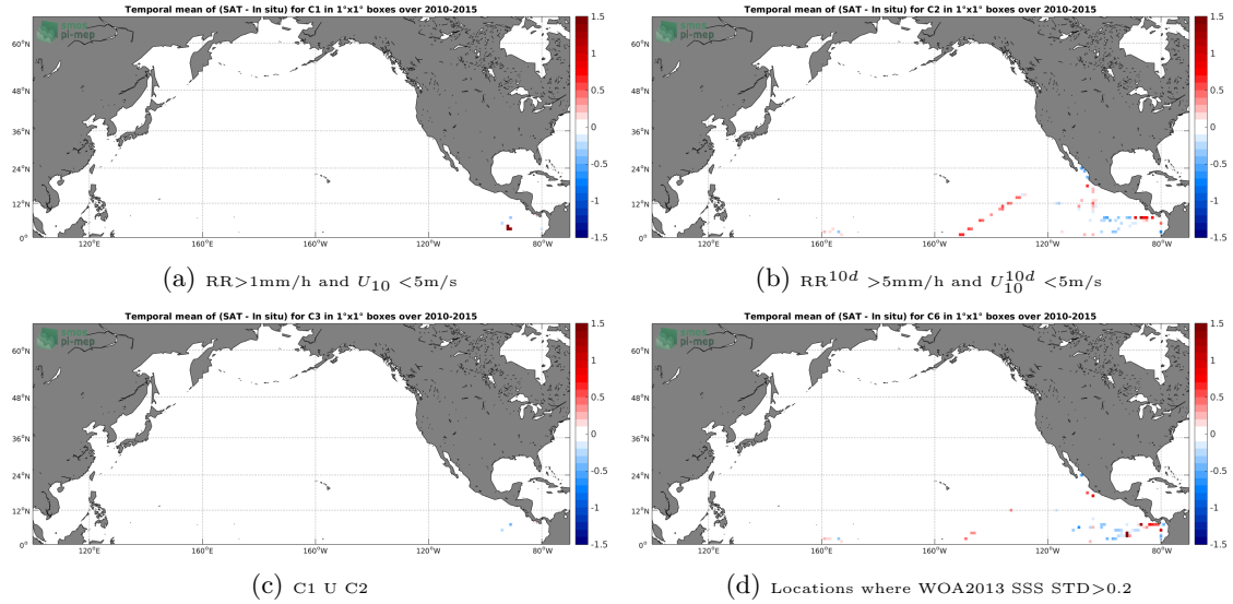
Figure 12: Temporal mean gridded over spatial boxes of size 1^\circ \times 1^\circ of \Delta SSS (SMOS-L4-CATDS-CECOS-IFREMER-V2-WEEKLY-0.5DEG - TSG-GOSUD-Research-vessel) for 4 different sub-datasets corresponding to: RR > 1\text{mm/h} and U_{10} < 5\text{m/s} (a), RR ^{10d} > 5\text{mm/h} and U_{10}^{10d} < 5\text{m/s} (b), C1 U C2 (c), Locations where WOA2013 SSS STD > 0.2 (d).
