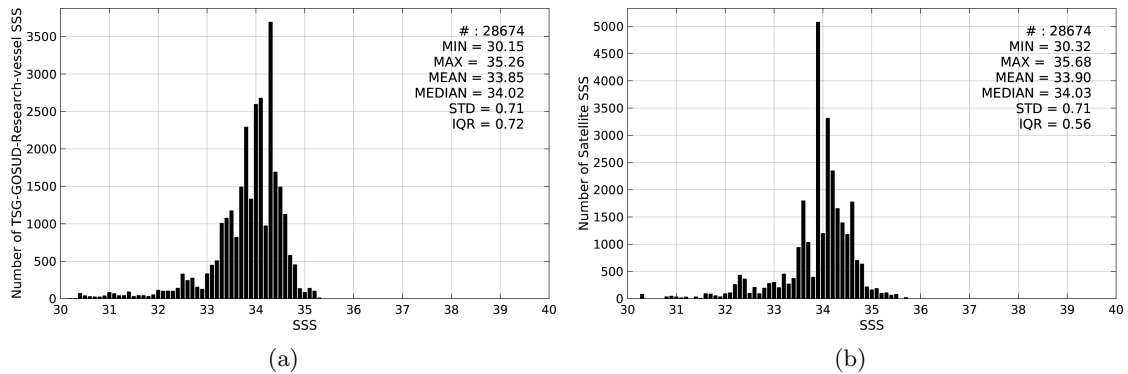
Figure 2: Histograms of SSS from TSG-GOSUD-Research-vessel (a) and SMOS-L4-CATDS-CECOS-IFREMER-V2-WEEKLY-0.5DEG (b) considering all match-up pairs per bins of 0.1 over the North Pacific Ocean Pi-MEP region and for the full satellite product period.
