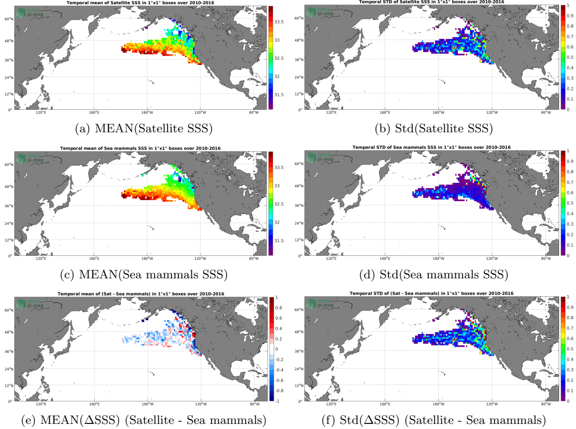
Figure 6: Temporal mean (left) and Std (right) of SSS from SMOS L4 v2 Weekly (CATDS-CECOS-IFREMER) (top), Sea mammals (middle), and of \Delta SSS (Satellite - Sea mammals). Only match-up pairs are used to generate these maps.
