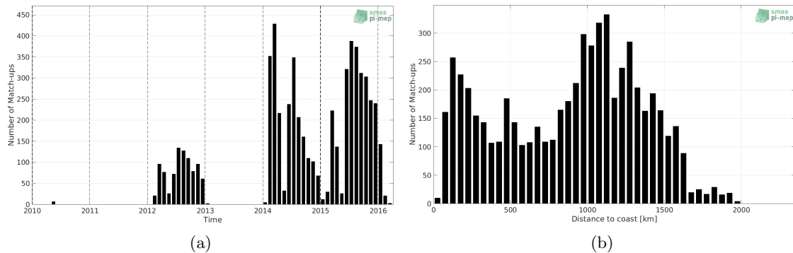
Figure 1: Number of match-ups between Sea mammals and SMOS L4 v2 Weekly (CATDS-CECOS-IFREMER) SSS as a function of time (a) and as function of the distance to coast (b) over the North Pacific Ocean Pi-MEP region and for the full satellite product period.
