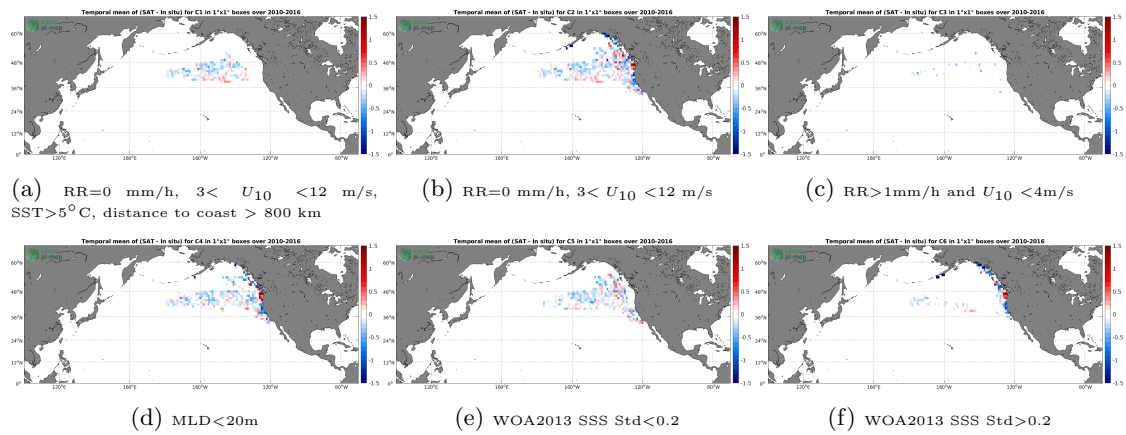
Figure 12: Temporal mean gridded over spatial boxes of size 1^\circ \times 1^\circ of \Delta SSS (SMOS L4 v2 Weekly (CATDS-CECOS-IFREMER) - Sea mammals) for 6 different subdatasets corresponding to:RR=0 mm/h, 3 < U_{10} < 12 m/s, SST >5^\circ\text{C} , distance to coast > 800 km (a), RR=0 mm/h, 3 < U_{10} < 12 m/s (b), RR >1 mm/h and U_{10} < 4 m/s (c),MLD <20 m (d),WOA2013 SSS Std <0.2 (e),WOA2013 SSS Std >0.2 (f).
