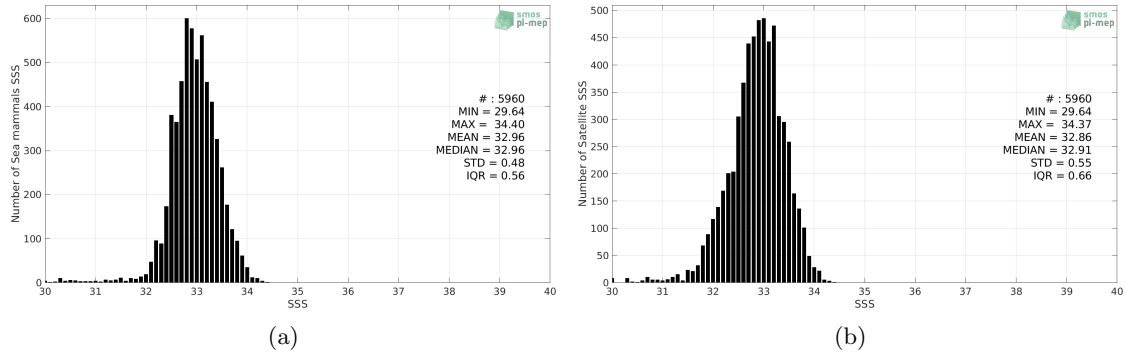
Figure 2: Histograms of SSS from Sea mammals (a) and SMOS L4 v2 Weekly (CATDS-CECOS-IFREMER) (b) considering all match-up pairs per bins of 0.1 over the North Pacific Ocean Pi-MEP region and for the full satellite product period.
