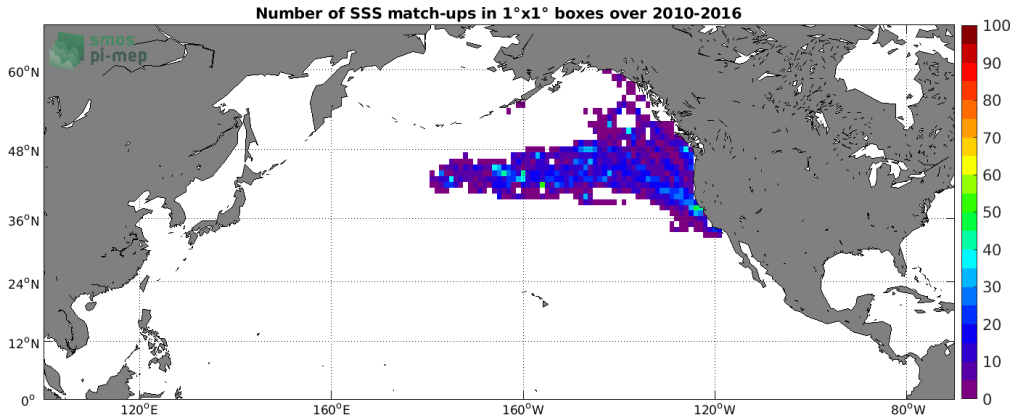
Figure 4: Number of SSS match-ups between Sea mammals SSS and the SMOS L4 v2 Weekly (CATDS-CECOS-IFREMER) SSS product for the North Pacific Ocean Pi-MEP region over 1^\circ \times 1^\circ boxes and for the full satellite product period.
