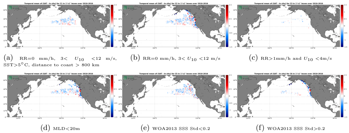
Figure 12: Temporal mean gridded over spatial boxes of size 1°x1° of \Delta SSS (SMOS L4 v2 Weekly (CATDS-CECOS-IFREMER) - Sea mammals) for 6 different subdatasets corresponding to:RR=0 mm/h, 3 < U_{10} < 12 m/s, SST>5°C, distance to coast > 800 km (a), RR=0 mm/h, 3 < U_{10} < 12 m/s (b), RR>1mm/h and U_{10} < 4 m/s (c),MLD<20m (d),WOA2013 SSS Std<0.2 (e),WOA2013 SSS Std>0.2 (f).
