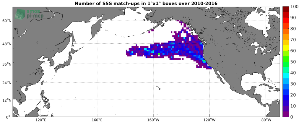
Figure 4: Number of SSS match-ups between Sea mammals SSS and the SMOS-L4-CATDS-CECOS-IFREMER-V2-WEEKLY-0.5DEG SSS product for the North Pacific Ocean Pi-MEP region over 1°x1° boxes and for the full satellite product period.
