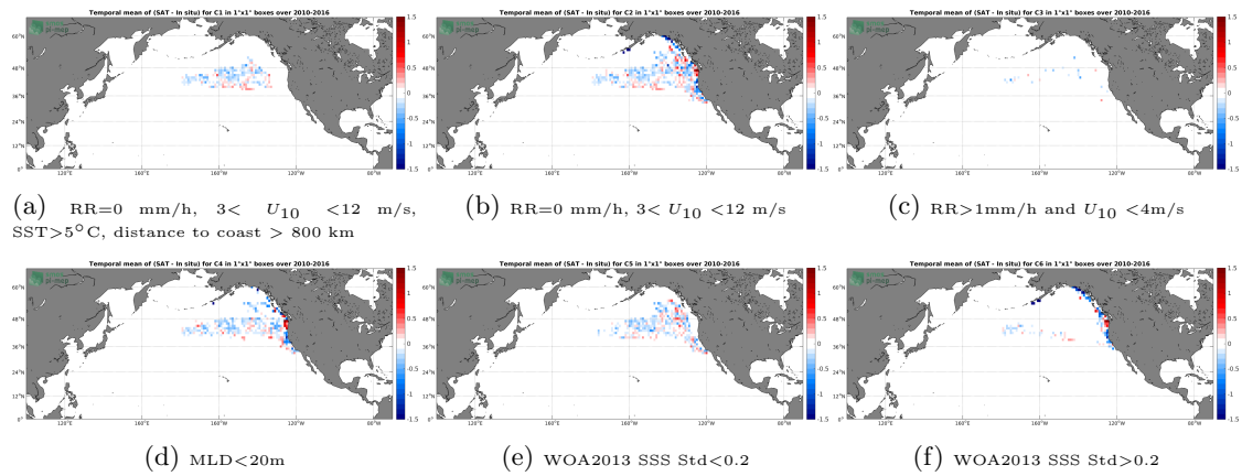
Figure 12: Temporal mean gridded over spatial boxes of size 1^{\circ}\times 1^{\circ} of \Delta\text{SSS} (SMOS-L4-CATDS-CECOS-IFREMER-V2-WEEKLY-0.5DEG - Sea mammals) for 6 different subdatasets corresponding to:RR=0 mm/h, 3 < U_{10} < 12 m/s, SST > 5^{\circ}\text{C} , distance to coast > 800 km (a), RR=0 mm/h, 3 < U_{10} < 12 m/s (b), RR > 1\text{mm/h} and U_{10} < 4\text{m/s} (c),MLD < 20\text{m} (d),WOA2013 SSS Std < 0.2 (e),WOA2013 SSS Std > 0.2 (f).
