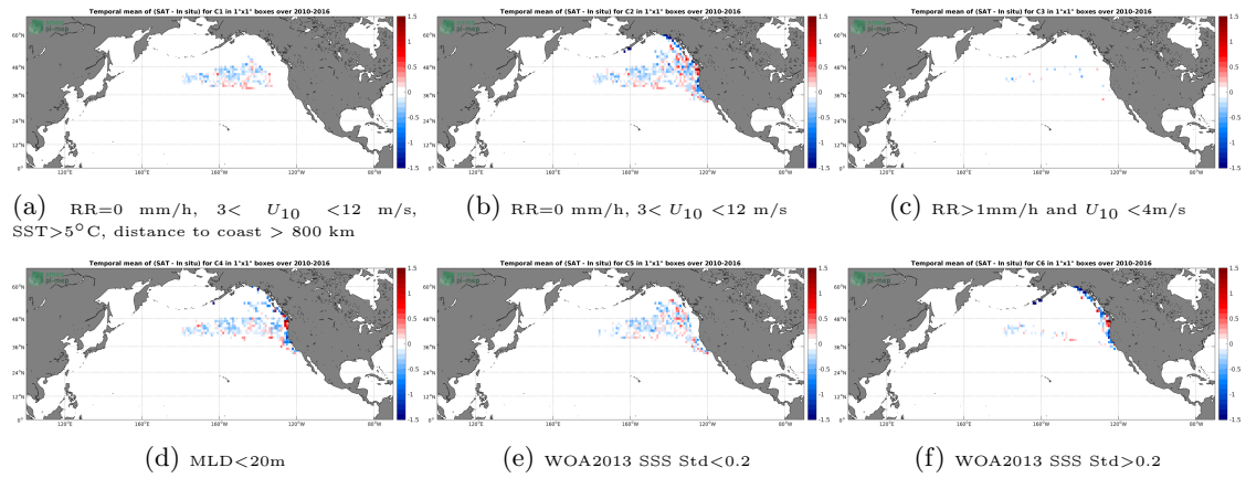
Figure 12: Temporal mean gridded over spatial boxes of size 1^\circ \times 1^\circ of \Delta SSS (SMOS-L4-CATDS-CECOS-IFREMER-V2-WEEKLY-0.5DEG - Sea mammals) for 6 different subdatasets corresponding to:RR=0 mm/h, 3 < U_{10} < 12 m/s, SST >5^\circ C, distance to coast > 800 km (a), RR=0 mm/h, 3 < U_{10} < 12 m/s (b), RR >1 mm/h and U_{10} < 4 m/s (c),MLD <20 m (d),WOA2013 SSS Std <0.2 (e),WOA2013 SSS Std >0.2 (f).
