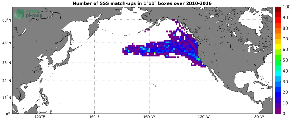
Figure 4: Number of SSS match-ups between Sea mammals SSS and the SMOS-L4-CATDS-CECOS-IFREMER-V2-WEEKLY-0.5DEG SSS product for the North Pacific Ocean Pi-MEP region over 1^\circ \times 1^\circ boxes and for the full satellite product period.
