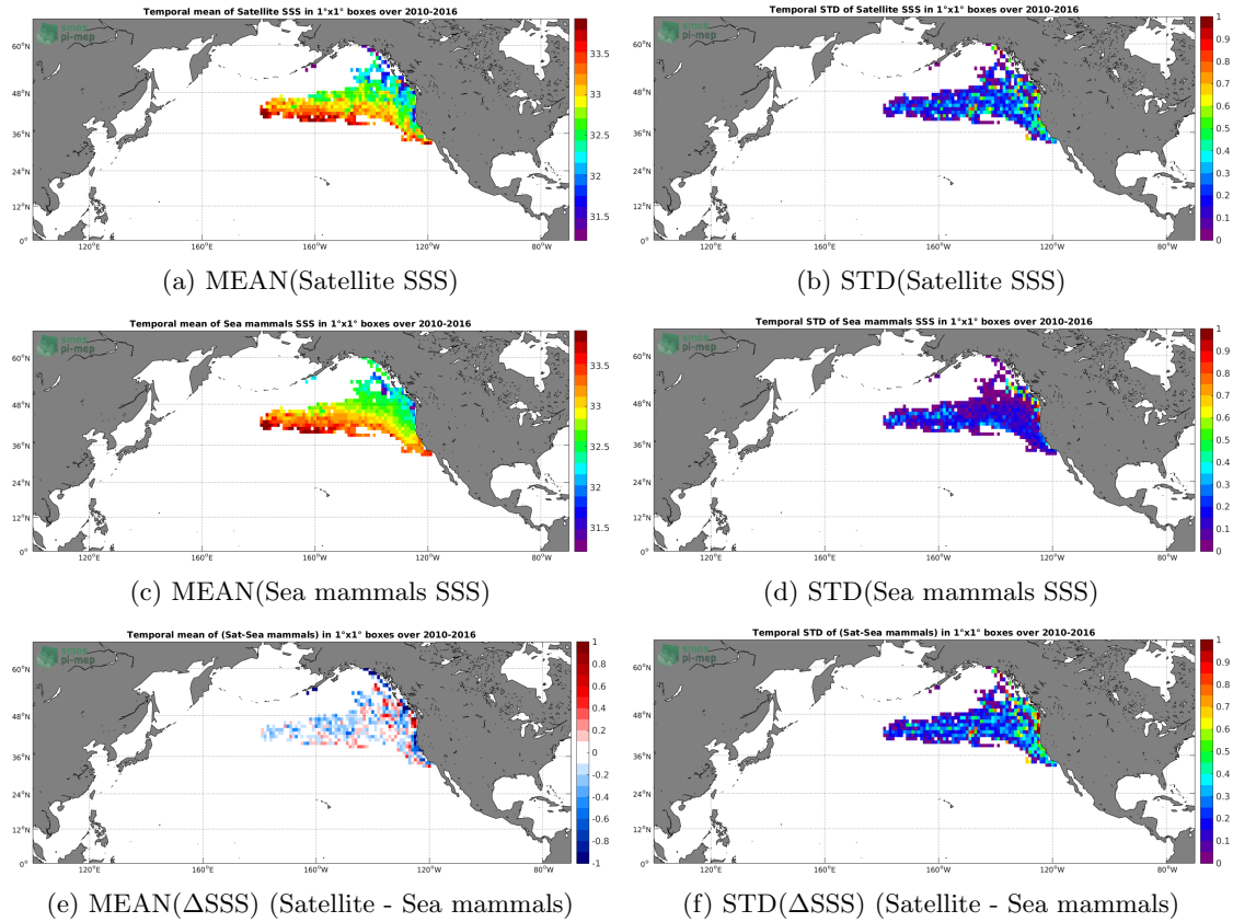
Figure 6: Temporal mean (left) and STD (right) of SSS from SMOS-L4-CATDS-CECOS-IFREMER-V2-WEEKLY-0.5DEG (top), Sea mammals (middle), and of \Delta SSS (Satellite - Sea mammals). Only match-up pairs are used to generate these maps.
