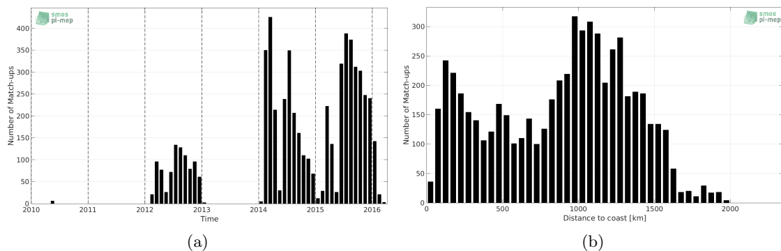
Figure 1: Number of match-ups between Sea mammals and SMOS-L4-CATDS-CECOS-IFREMER-V2-WEEKLY-0.5DEG SSS as a function of time (a) and as function of the distance to coast (b) over the North Pacific Ocean Pi-MEP region and for the full satellite product period.
