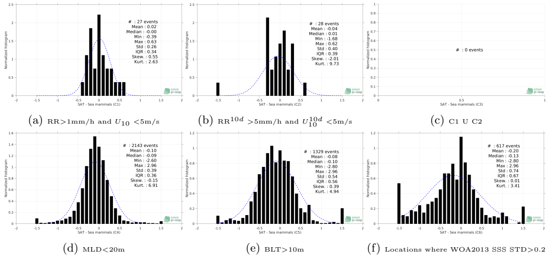
Figure 13: Normalized histogram of ΔSSS (SMOS-L4-CATDS-CECOS-IFREMER-V2-WEEKLY-0.5DEG - Sea mammals) for 6 different subdatasets corresponding to: RR>1mm/h and U_{10} < 5\text{m/s} (a), RR^{10d} > 5\text{mm/h} and U_{10}^{10d} < 5\text{m/s} (b), C1 U C2 (c),MLD<20m (d),BLT>10m (e),Locations where WOA2013 SSS STD>0.2 (f).
