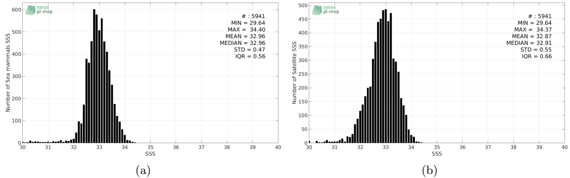
Figure 2: Histograms of SSS from Sea mammals (a) and SMOS-L4-CATDS-CECOS-IFREMER-V2-WEEKLY-0.5DEG (b) considering all match-up pairs per bins of 0.1 over the North Pacific Ocean Pi-MEP region and for the full satellite product period.
