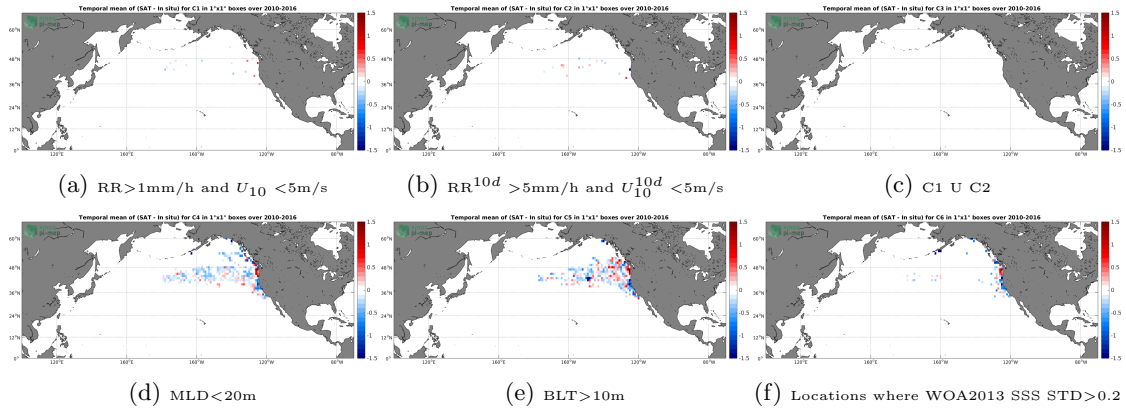
Figure 12: Temporal mean gridded over spatial boxes of size 1°x1° of ΔSSS (SMOS-L4-CATDS-CECOS-IFREMER-V2-WEEKLY-0.5DEG - Sea mammals) for 6 different subdatasets corresponding to:RR>1mm/h and U_{10} < 5\text{m/s} (a), RR^{10d} > 5\text{mm/h} and U_{10}^{10d} < 5\text{m/s} (b), C1 U C2 (c),MLD<20m (d),BLT>10m (e),Locations where WOA2013 SSS STD>0.2 (f).
