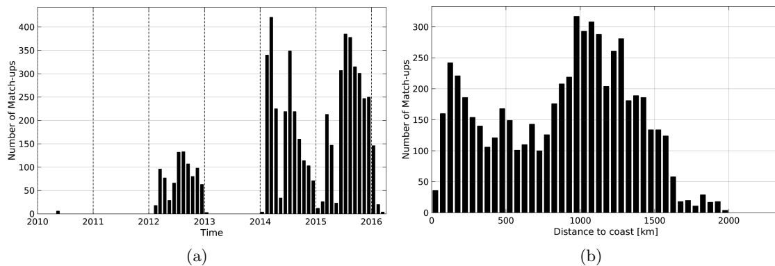
Figure 1: Number of match-ups between Sea mammals and SMOS-L4-CATDS-CECOS-IFREMER-V2-WEEKLY-0.5DEG SSS as a function of time (a) and as function of the distance to coast (b) over the North Pacific Ocean Pi-MEP region and for the full satellite product period.
