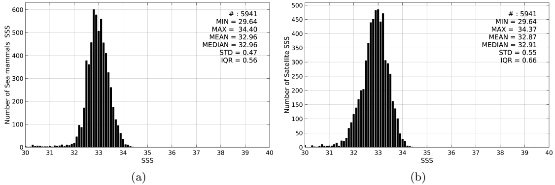
Figure 2: Histograms of SSS from Sea mammals (a) and SMOS-L4-CATDS-CECOS-IFREMER-V2-WEEKLY-0.5DEG (b) considering all match-up pairs per bins of 0.1 over the North Pacific Ocean Pi-MEP region and for the full satellite product period.
