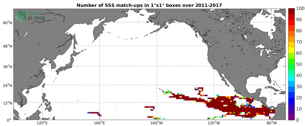
Figure 3: Number of SSS match-ups between Surface drifters SSS and the SMOS-L4-CATDS-CECOS-IFREMER-V2-WEEKLY-0.5DEG SSS product for the North Pacific Ocean Pi-MEP region over 1^\circ \times 1^\circ boxes and for the full satellite product period.
