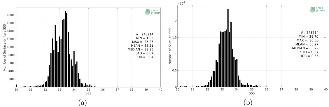
Figure 2: Histograms of SSS from Surface drifters (a) and SMOS-L4-CATDS-CECOS-IFREMER-V2-WEEKLY-0.5DEG (b) considering all match-up pairs per bins of 0.1 over the North Pacific Ocean Pi-MEP region and for the full satellite product period.
