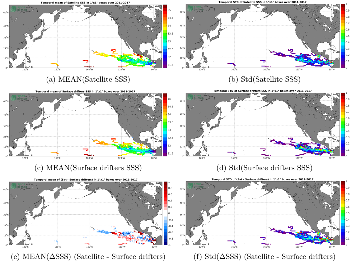
Figure 5: Temporal mean (left) and Std (right) of SSS from SMOS-L4-CATDS-CECOS-IFREMER-V2-WEEKLY-0.5DEG (top), Surface drifters (middle), and of \Delta SSS (Satellite - Surface drifters). Only match-up pairs are used to generate these maps.
