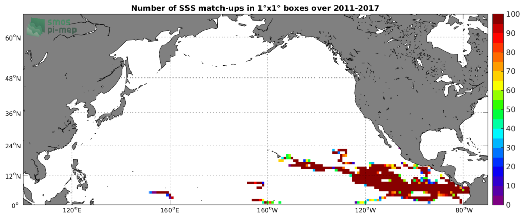
Figure 3: Number of SSS match-ups between Surface drifters SSS and the SMOS-L4-CATDS-CECOS-IFREMER-V2-WEEKLY-0.5DEG SSS product for the North Pacific Ocean Pi-MEP region over 1°x1° boxes and for the full satellite product period.
