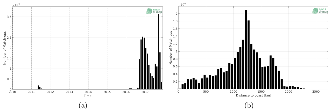
Figure 1: Number of match-ups between Surface drifters and SMOS-L4-CATDS-CECOS-IFREMER-V2-WEEKLY-0.5DEG SSS as a function of time (a) and as function of the distance to coast (b) over the North Pacific Ocean Pi-MEP region and for the full satellite product period.
