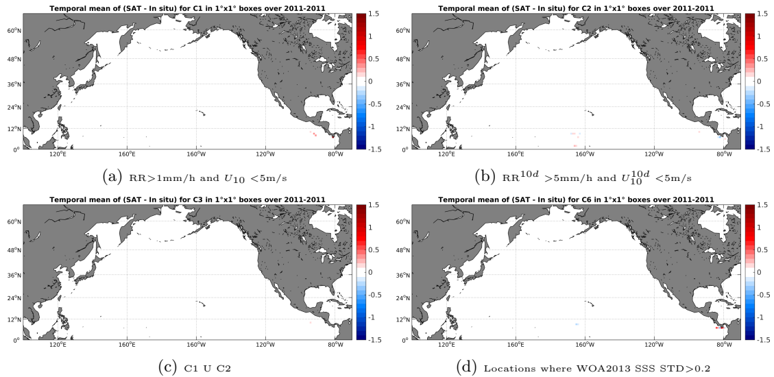
Figure 11: Temporal mean gridded over spatial boxes of size 1^\circ \times 1^\circ of \Delta SSS (SMOS-L4-CATDS-CECOS-IFREMER-V2-WEEKLY-0.5DEG - Surface drifters) for 4 different subdatasets corresponding to: RR > 1\text{mm/h} and U_{10} < 5\text{m/s} (a), RR^{10d} > 5\text{mm/h} and U_{10}^{10d} < 5\text{m/s} (b), C1 \cup C2 (c), Locations where WOA2013 SSS STD > 0.2 (d).
