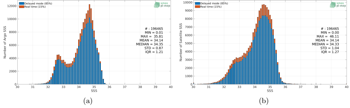
Figure 2: Histograms of SSS from Argo (a) and SMOS L4 v2 Weekly (CATDS-CECOS-IFREMER) (b) considering all match-up pairs per bins of 0.1 over the North Pacific Ocean Pi-MEP region and for the full satellite product period.
