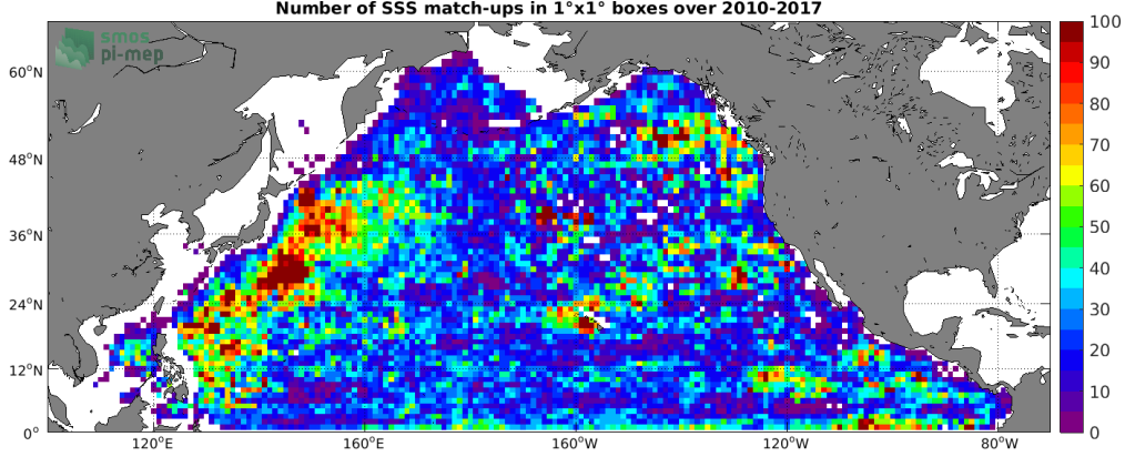
Figure 4: Number of SSS match-ups between Argo SSS and the SMOS L4 v2 Weekly (CATDS-CECOS-IFREMER) SSS product for the North Pacific Ocean Pi-MEP region over 1^\circ \times 1^\circ boxes and for the full satellite product period.
