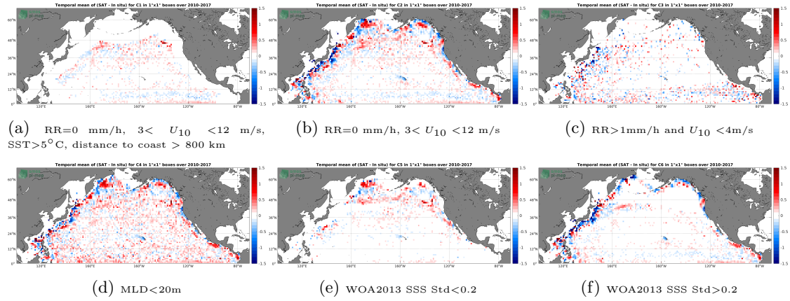
Figure 12: Temporal mean gridded over spatial boxes of size 1^\circ \times 1^\circ of \Delta SSS (SMOS L4 v2 Weekly (CATDS-CECOS-IFREMER) - Argo) for 6 different subdatasets corresponding to: RR=0 mm/h, 3 < U_{10} < 12 m/s, SST > 5^\circ C , distance to coast > 800 km (a), RR=0 mm/h, 3 < U_{10} < 12 m/s (b), RR > 1 mm/h and U_{10} < 4 m/s (c), MLD < 20 m (d), WOA2013 SSS Std < 0.2 (e), WOA2013 SSS Std > 0.2 (f).
