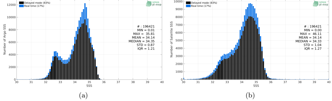
Figure 2: Histograms of SSS from Argo (a) and SMOS L4 v2 Weekly (CATDS-CECOS-IFREMER) (b) considering all match-up pairs per bins of 0.1 over the North Pacific Ocean Pi-MEP region and for the full satellite product period.
