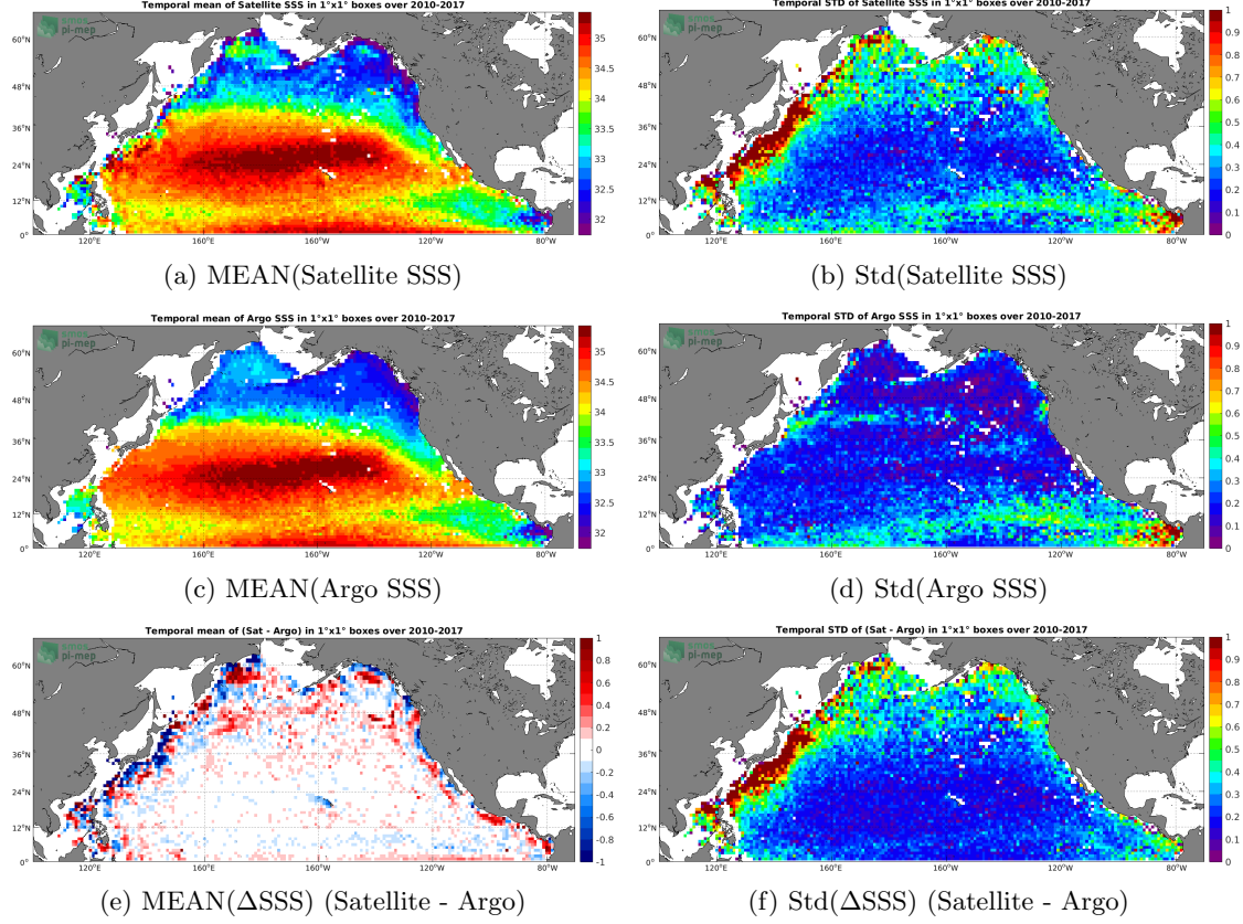
Figure 6: Temporal mean (left) and Std (right) of SSS from SMOS L4 v2 Weekly (CATDS-CECOS-IFREMER) (top), Argo (middle), and of \Delta SSS (Satellite - Argo). Only match-up pairs are used to generate these maps.
