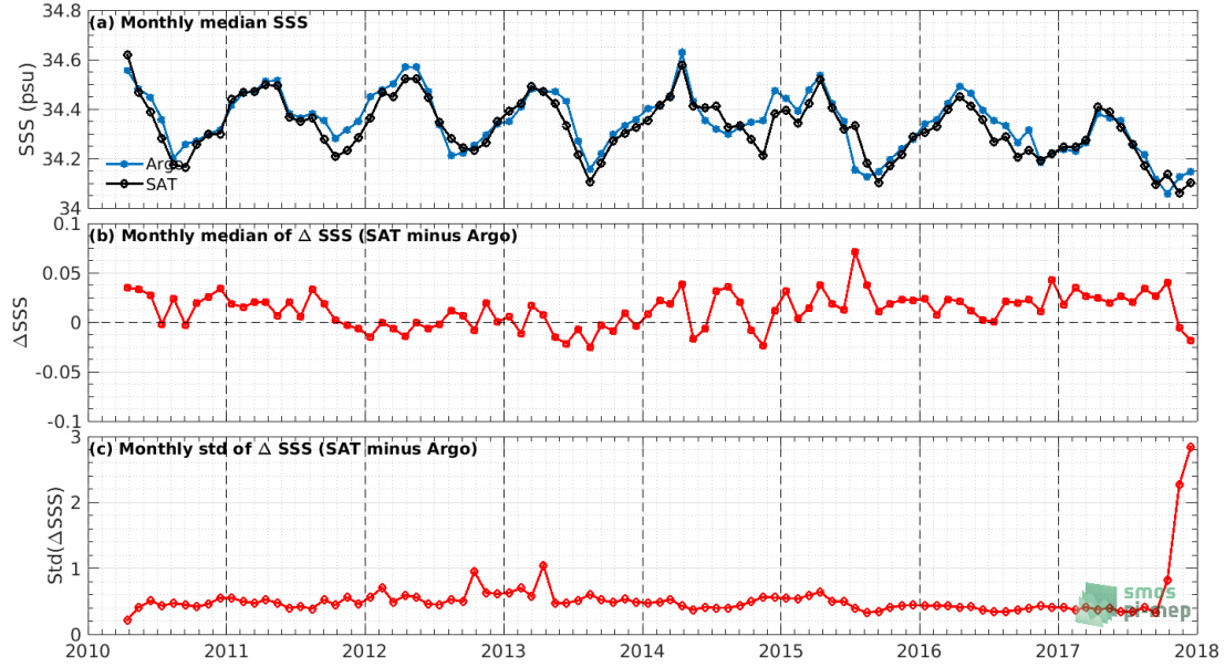
Figure 7: Time series of the monthly median SSS (top), median of \Delta\text{SSS} (Satellite - Argo) and Std of \Delta\text{SSS} (Satellite - Argo) over the North Pacific Ocean Pi-MEP region considering all match-ups collected by the Pi-MEP.
