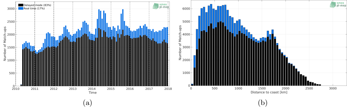
Figure 1: Number of match-ups between Argo and SMOS L4 v2 Weekly (CATDS-CECOS-IFREMER) SSS as a function of time (a) and as function of the distance to coast (b) over the North Pacific Ocean Pi-MEP region and for the full satellite product period.
