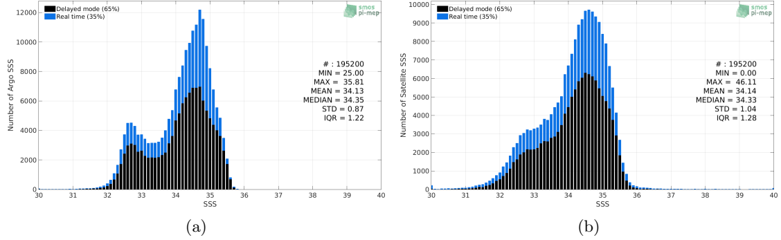
Figure 2: Histograms of SSS from Argo (a) and SMOS-L4-CATDS-CECOS-IFREMER-V2-WEEKLY-0.5DEG (b) considering all match-up pairs per bins of 0.1 over the North Pacific Ocean Pi-MEP region and for the full satellite product period.
