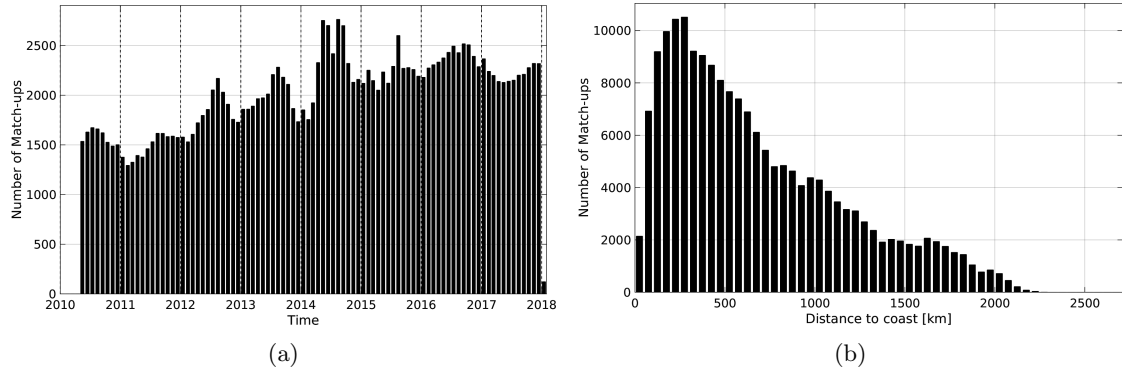
Figure 1: Number of match-ups between Argo and SMOS-L4-CATDS-CECOS-IFREMER-V2-WEEKLY-0.5DEG SSS as a function of time (a) and as function of the distance to coast (b) over the North Pacific Ocean Pi-MEP region and for the full satellite product period.
