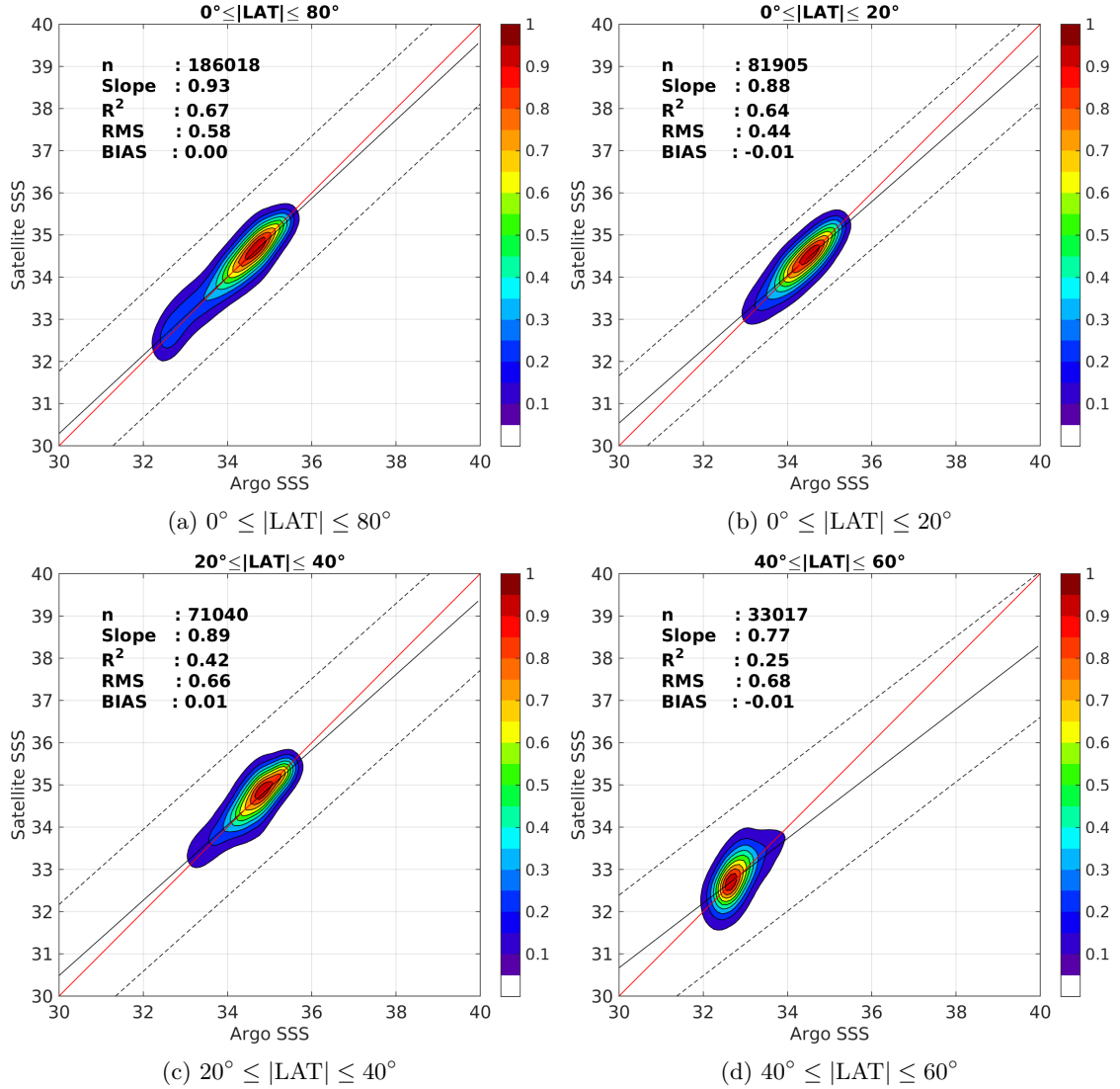
Figure 9: Contour maps of the concentration of SMOS-L4-CATDS-CECOS-IFREMER-V2-WEEKLY-0.5DEG SSS (y-axis) versus Argo SSS (x-axis) at match-up pairs for different latitude bands. For each plot, the red line shows x=y . The black thin and dashed lines indicate a linear fit through the data cloud and the \pm 95\% confidence levels, respectively. The number match-up pairs n , the slope and R^2 coefficient of the linear fit, the root mean square (RMS) and the mean bias between satellite and in situ data are indicated for each latitude band in each plots.
