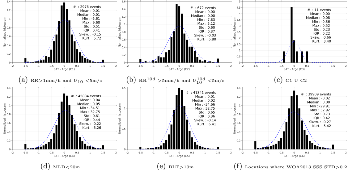
Figure 13: Normalized histogram of \Delta SSS (SMOS-L4-CATDS-CECOS-IFREMER-V2-WEEKLY-0.5DEG - Argo) for 6 different subdatasets corresponding to: RR > 1\text{mm/h} and U_{10} < 5\text{m/s} (a), RR^{10d} > 5\text{mm/h} and U_{10}^{10d} < 5\text{m/s} (b), C1 \cup C2 (c), MLD < 20\text{m} (d), BLT > 10\text{m} (e), Locations where WOA2013 SSS STD > 0.2 (f).
