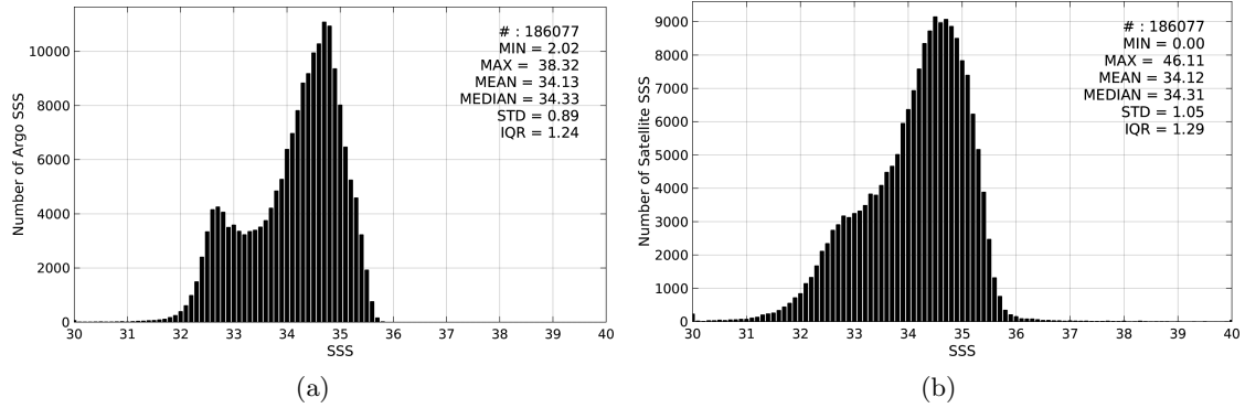
Figure 2: Histograms of SSS from Argo (a) and SMOS-L4-CATDS-CECOS-IFREMER-V2-WEEKLY-0.5DEG (b) considering all match-up pairs per bins of 0.1 over the North Pacific Ocean Pi-MEP region and for the full satellite product period.
