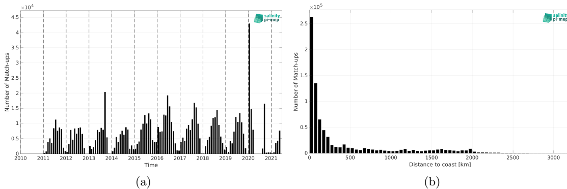
Figure 2: Number of match-ups between TSG (SAMOS) and SMOS SSS L4 v2 - Daily (BEC) SSS as a function of time (a) and as function of the distance to coast (b) over the North Pacific Ocean Pi-MEP region and for the full satellite product period.
