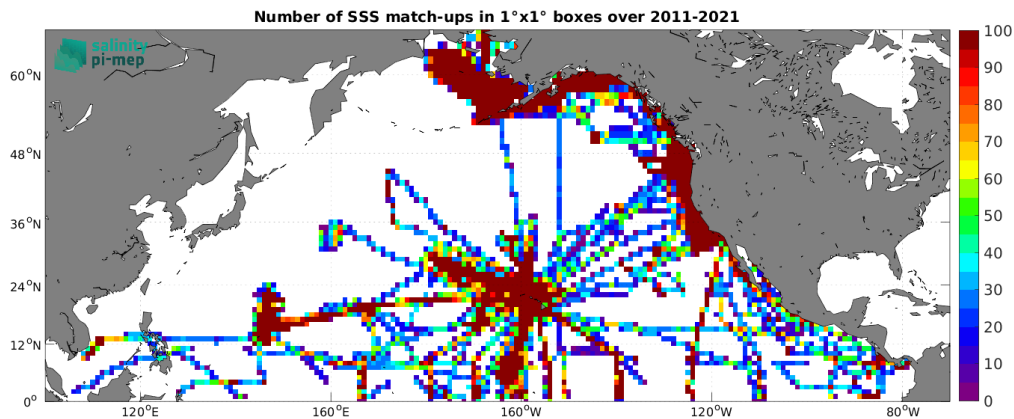
Figure 5: Number of SSS match-ups between TSG (SAMOS) SSS and the SMOS SSS L4 v2 - Daily (BEC) SSS product for the North Pacific Ocean Pi-MEP region over 1^\circ \times 1^\circ boxes and for the full satellite product period.
