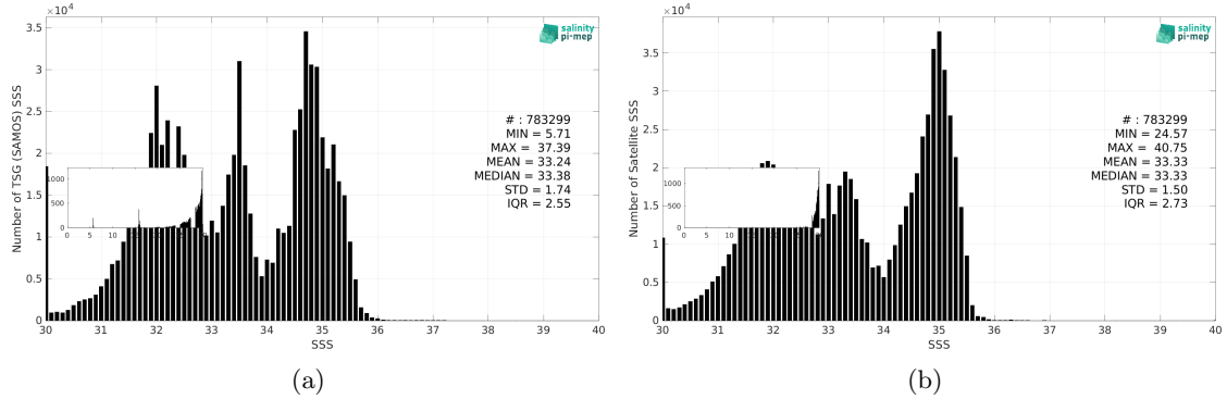
Figure 3: Histograms of SSS from TSG (SAMOS) (a) and SMOS SSS L4 v2 - Daily (BEC) (b) considering all match-up pairs per bins of 0.1 over the North Pacific Ocean Pi-MEP region and for the full satellite product period.
