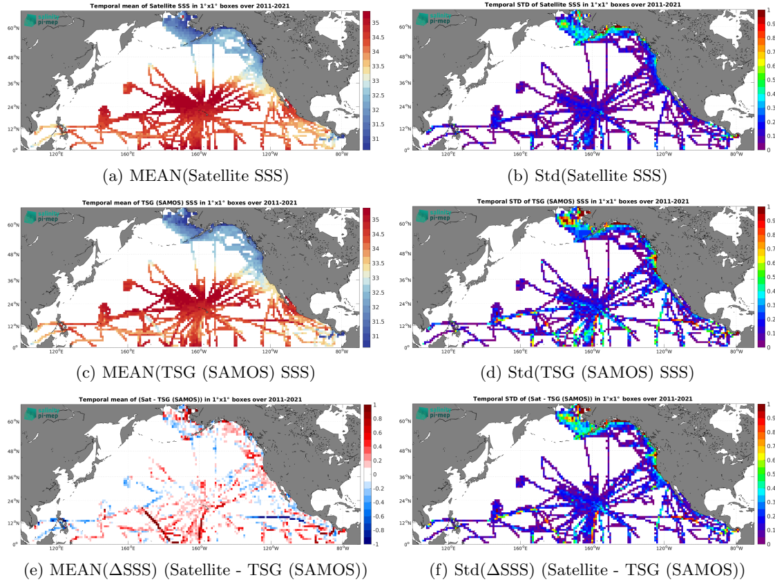
Figure 7: Temporal mean (left) and Std (right) of SSS from SMOS SSS L4 v2 - Daily (BEC) (top), TSG (SAMOS) (middle), and of \Delta\text{SSS} (Satellite - TSG (SAMOS)). Only match-up pairs are used to generate these maps.
