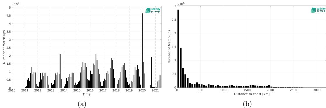
Figure 1: Number of match-ups between TSG (SAMOS) and SMOS SSS L4 v2 - Daily (BEC) SSS as a function of time (a) and as function of the distance to coast (b) over the North Pacific Ocean Pi-MEP region and for the full satellite product period.
