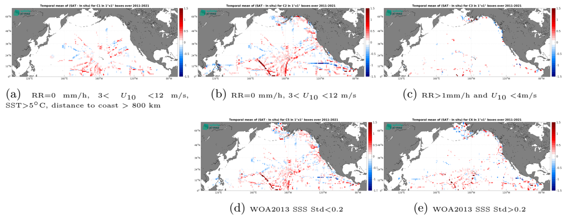
Figure 12: Temporal mean gridded over spatial boxes of size 1^\circ \times 1^\circ of \Delta SSS (SMOS SSS L4 v2 - Daily (BEC) - TSG (SAMOS)) for 5 different subdatasets corresponding to:RR=0 mm/h, 3 < U_{10} < 12 m/s, SST >5^\circ\text{C} , distance to coast > 800 km (a), RR=0 mm/h, 3 < U_{10} < 12 m/s (b), RR >1 mm/h and U_{10} < 4 m/s (c), WOA2013 SSS Std <0.2 (d), WOA2013 SSS Std >0.2 (e).
