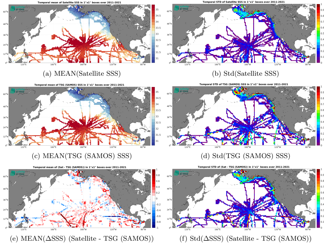
Figure 6: Temporal mean (left) and Std (right) of SSS from SMOS SSS L4 v2 - Daily (BEC) (top), TSG (SAMOS) (middle), and of \Delta\text{SSS} (Satellite - TSG (SAMOS)). Only match-up pairs are used to generate these maps.
