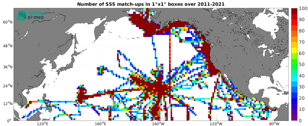
Figure 4: Number of SSS match-ups between TSG (SAMOS) SSS and the SMOS SSS L4 v2 - Daily (BEC) SSS product for the North Pacific Ocean Pi-MEP region over 1^\circ \times 1^\circ boxes and for the full satellite product period.
