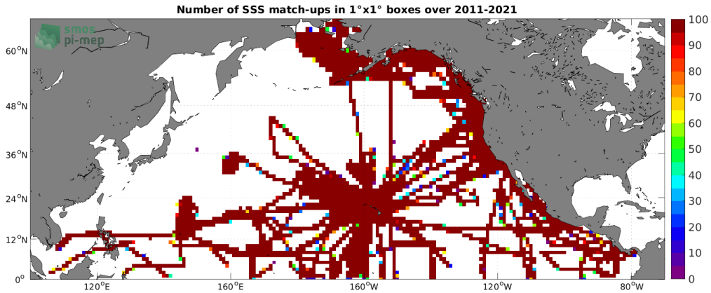
Figure 4: Number of SSS match-ups between TSG (SAMOS) SSS and the SMOS SSS L4 v2 - Daily (BEC) SSS product for the North Pacific Ocean Pi-MEP region over 1°x1° boxes and for the full satellite product period.
