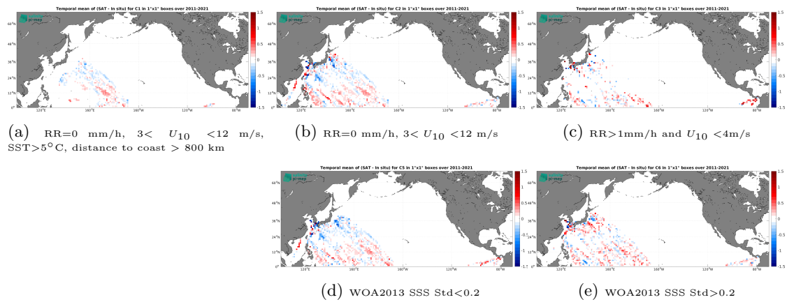
Figure 14: Temporal mean gridded over spatial boxes of size 1^\circ \times 1^\circ of \Delta\text{SSS} (SMOS SSS L4 v2 - Daily (BEC) - TSG (LEGOS-DM)) for 5 different subdatasets corresponding to: RR=0 mm/h, 3 < U_{10} < 12 m/s, SST > 5°C, distance to coast > 800 km (a), RR=0 mm/h, 3 < U_{10} < 12 m/s (b), RR > 1mm/h and U_{10} < 4 m/s (c), WOA2013 SSS Std < 0.2 (d), WOA2013 SSS Std > 0.2 (e).
