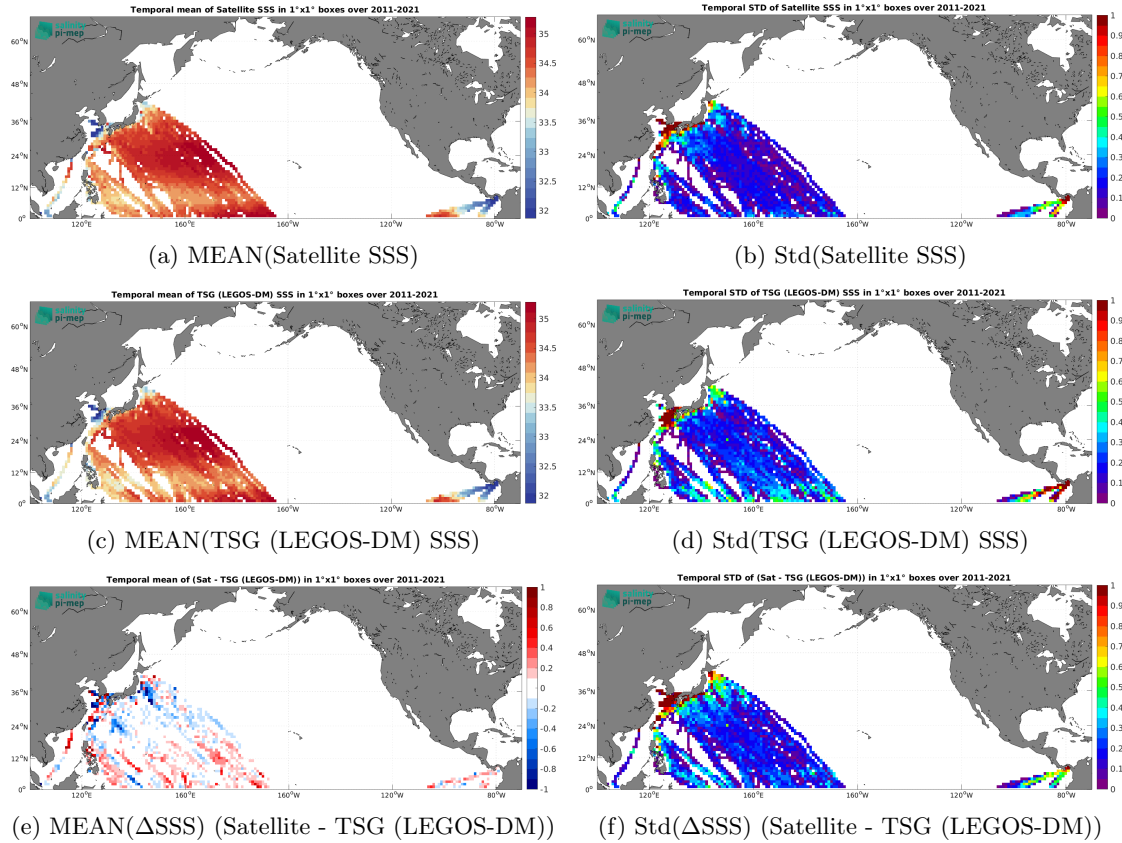
Figure 7: Temporal mean (left) and Std (right) of SSS from SMOS SSS L4 v2 - Daily (BEC) (top), TSG (LEGOS-DM) (middle), and of \Delta\text{SSS} (Satellite - TSG (LEGOS-DM)). Only match-up pairs are used to generate these maps.
