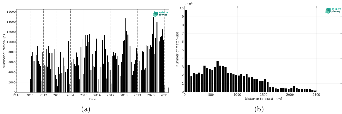
Figure 1: Number of match-ups between TSG (LEGOS-DM) and SMOS SSS L4 v2 - Daily (BEC) SSS as a function of time (a) and as function of the distance to coast (b) over the North Pacific Ocean Pi-MEP region and for the full satellite product period.
