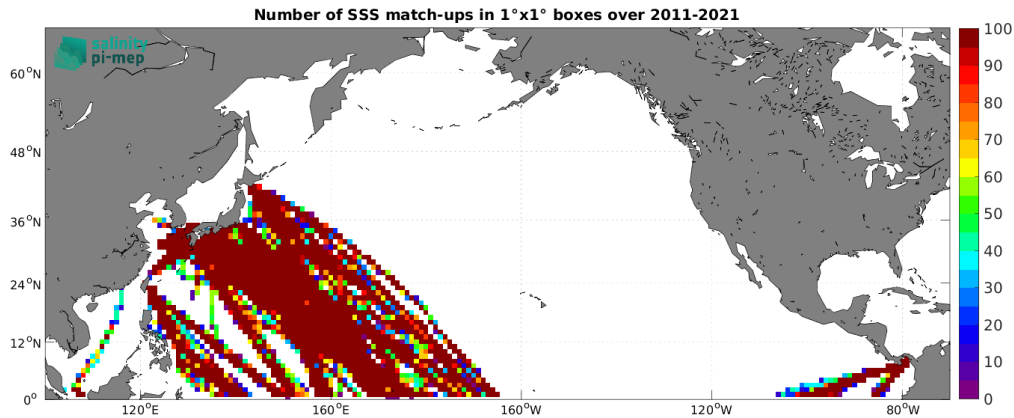
Figure 4: Number of SSS match-ups between TSG (LEGOS-DM) SSS and the SMOS SSS L4 v2 - Daily (BEC) SSS product for the North Pacific Ocean Pi-MEP region over 1^\circ \times 1^\circ boxes and for the full satellite product period.
