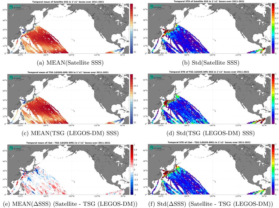
Figure 6: Temporal mean (left) and Std (right) of SSS from SMOS SSS L4 v2 - Daily (BEC) (top), TSG (LEGOS-DM) (middle), and of \Delta\text{SSS} (Satellite - TSG (LEGOS-DM)). Only match-up pairs are used to generate these maps.
