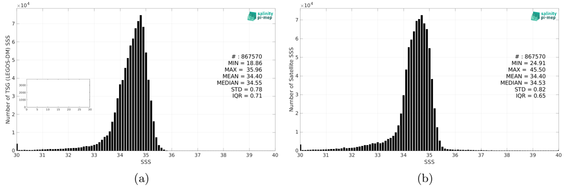
Figure 2: Histograms of SSS from TSG (LEGOS-DM) (a) and SMOS SSS L4 v2 - Daily (BEC) (b) considering all match-up pairs per bins of 0.1 over the North Pacific Ocean Pi-MEP region and for the full satellite product period.
