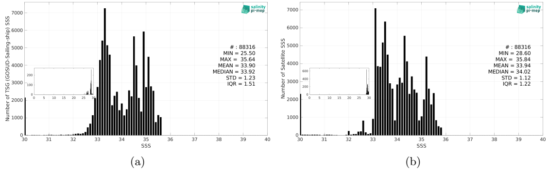
Figure 3: Histograms of SSS from TSG (GOSUD-Sailing-ship) (a) and SMOS SSS L4 v2 - Daily (BEC) (b) considering all match-up pairs per bins of 0.1 over the North Pacific Ocean Pi-MEP region and for the full satellite product period.
