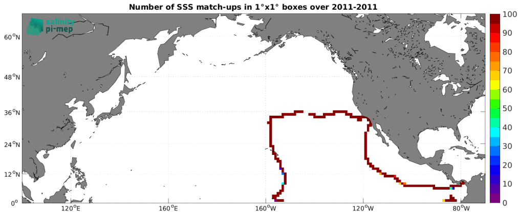
Figure 4: Number of SSS match-ups between TSG (GOSUD-Sailing-ship) SSS and the SMOS SSS L4 v2 - Daily (BEC) SSS product for the North Pacific Ocean Pi-MEP region over 1^\circ \times 1^\circ boxes and for the full satellite product period.
