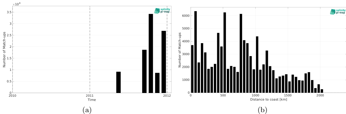
Figure 1: Number of match-ups between TSG (GOSUD-Sailing-ship) and SMOS SSS L4 v2 - Daily (BEC) SSS as a function of time (a) and as function of the distance to coast (b) over the North Pacific Ocean Pi-MEP region and for the full satellite product period.
