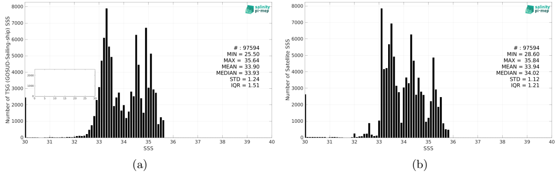
Figure 2: Histograms of SSS from TSG (GOSUD-Sailing-ship) (a) and SMOS SSS L4 v2 - Daily (BEC) (b) considering all match-up pairs per bins of 0.1 over the North Pacific Ocean Pi-MEP region and for the full satellite product period.
