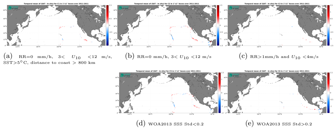
Figure 12: Temporal mean gridded over spatial boxes of size 1^\circ \times 1^\circ of \Delta\text{SSS} (SMOS SSS L4 v2 - Daily (BEC) - TSG (GOSUD-Sailing-ship)) for 5 different subdatasets corresponding to:RR=0 mm/h, 3 < U_{10} < 12 m/s, SST >5^\circ\text{C} , distance to coast > 800 km (a), RR=0 mm/h, 3 < U_{10} < 12 m/s (b), RR >1 mm/h and U_{10} < 4 m/s (c), WOA2013 SSS Std <0.2 (d), WOA2013 SSS Std >0.2 (e).
