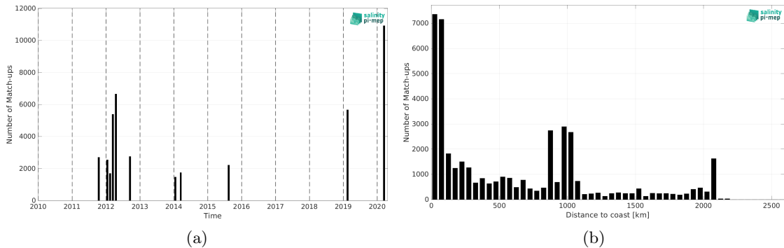
Figure 2: Number of match-ups between TSG (GOSUD-Research-vessel) and SMOS SSS L4 v2 - Daily (BEC) SSS as a function of time (a) and as function of the distance to coast (b) over the North Pacific Ocean Pi-MEP region and for the full satellite product period.
