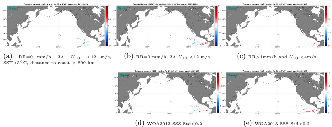
Figure 14: Temporal mean gridded over spatial boxes of size 1^\circ \times 1^\circ of \Delta SSS (SMOS SSS L4 v2 - Daily (BEC) - TSG (GOSUD-Research-vessel)) for 5 different subdatasets corresponding to: RR=0 mm/h, 3 < U_{10} < 12 m/s, SST > 5°C, distance to coast > 800 km (a), RR=0 mm/h, 3 < U_{10} < 12 m/s (b), RR > 1 mm/h and U_{10} < 4 m/s (c), WOA2013 SSS Std < 0.2 (d), WOA2013 SSS Std > 0.2 (e).
