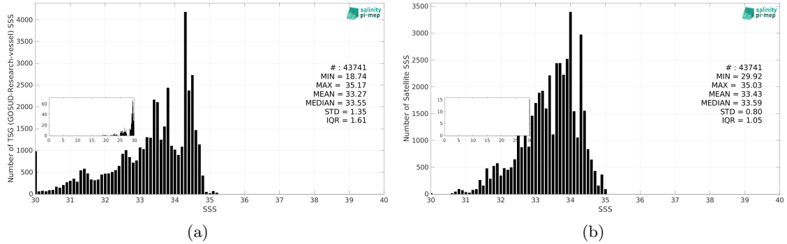
Figure 3: Histograms of SSS from TSG (GOSUD-Research-vessel) (a) and SMOS SSS L4 v2 - Daily (BEC) (b) considering all match-up pairs per bins of 0.1 over the North Pacific Ocean Pi-MEP region and for the full satellite product period.
