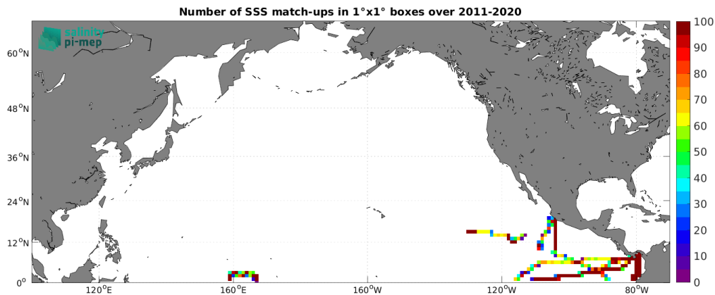
Figure 5: Number of SSS match-ups between TSG (GOSUD-Research-vessel) SSS and the SMOS SSS L4 v2 - Daily (BEC) SSS product for the North Pacific Ocean Pi-MEP region over 1^\circ \times 1^\circ boxes and for the full satellite product period.
