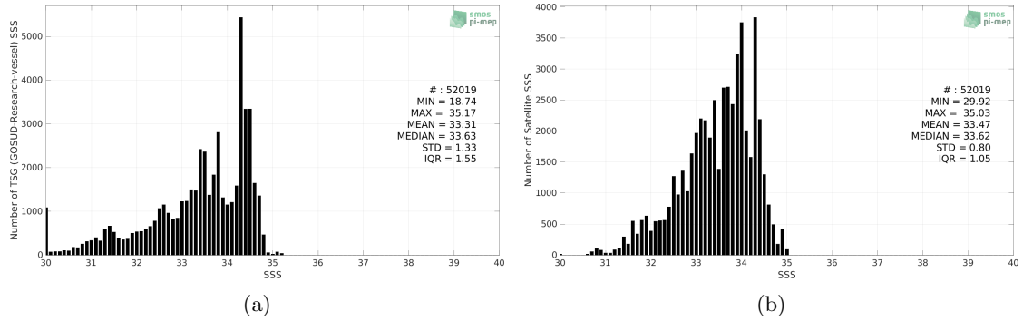
Figure 2: Histograms of SSS from TSG (GOSUD-Research-vessel) (a) and SMOS SSS L4 v2 - Daily (BEC) (b) considering all match-up pairs per bins of 0.1 over the North Pacific Ocean Pi-MEP region and for the full satellite product period.
