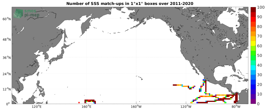
Figure 4: Number of SSS match-ups between TSG (GOSUD-Research-vessel) SSS and the SMOS SSS L4 v2 - Daily (BEC) SSS product for the North Pacific Ocean Pi-MEP region over 1^\circ \times 1^\circ boxes and for the full satellite product period.
