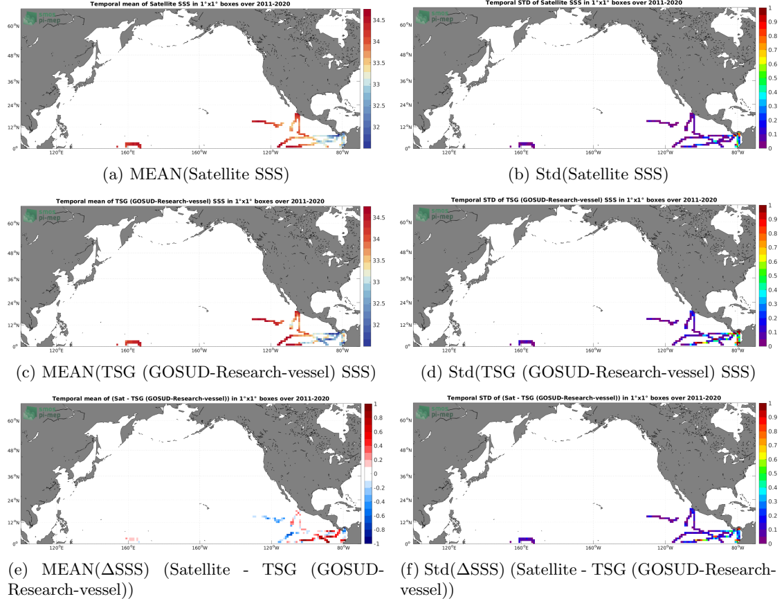
Figure 6: Temporal mean (left) and Std (right) of SSS from SMOS SSS L4 v2 - Daily (BEC) (top), TSG (GOSUD-Research-vessel) (middle), and of \Delta SSS (Satellite - TSG (GOSUD-Research-vessel)). Only match-up pairs are used to generate these maps.
