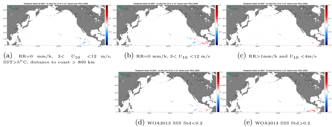
Figure 12: Temporal mean gridded over spatial boxes of size 1^\circ \times 1^\circ of \Delta\text{SSS} (SMOS SSS L4 v2 - Daily (BEC) - TSG (GOSUD-Research-vessel)) for 5 different subdatasets corresponding to:RR=0 mm/h, 3 < U_{10} < 12 m/s, SST >5^\circ\text{C} , distance to coast > 800 km (a), RR=0 mm/h, 3 < U_{10} < 12 m/s (b), RR >1 mm/h and U_{10} < 4 m/s (c), WOA2013 SSS Std <0.2 (d), WOA2013 SSS Std >0.2 (e).
