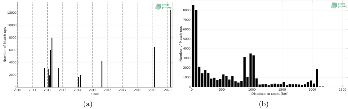
Figure 1: Number of match-ups between TSG (GOSUD-Research-vessel) and SMOS SSS L4 v2 - Daily (BEC) SSS as a function of time (a) and as function of the distance to coast (b) over the North Pacific Ocean Pi-MEP region and for the full satellite product period.
