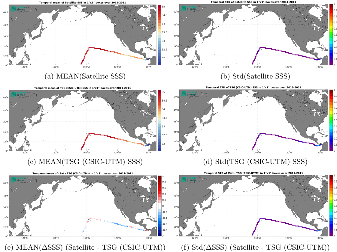
Figure 6: Temporal mean (left) and Std (right) of SSS from SMOS SSS L4 v2 - Daily (BEC) (top), TSG (CSIC-UTM) (middle), and of \Delta\text{SSS} (Satellite - TSG (CSIC-UTM)). Only match-up pairs are used to generate these maps.
