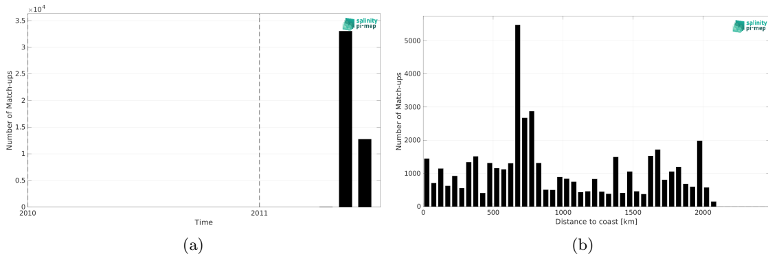
Figure 1: Number of match-ups between TSG (CSIC-UTM) and SMOS SSS L4 v2 - Daily (BEC) SSS as a function of time (a) and as function of the distance to coast (b) over the North Pacific Ocean Pi-MEP region and for the full satellite product period.
