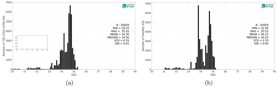
Figure 2: Histograms of SSS from TSG (CSIC-UTM) (a) and SMOS SSS L4 v2 - Daily (BEC) (b) considering all match-up pairs per bins of 0.1 over the North Pacific Ocean Pi-MEP region and for the full satellite product period.
