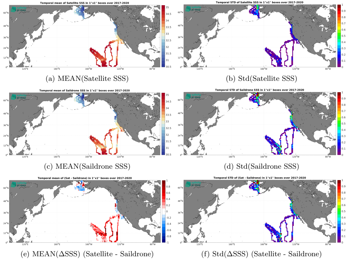
Figure 7: Temporal mean (left) and Std (right) of SSS from SMOS SSS L4 v2 - Daily (BEC) (top), Saildrone (middle), and of \Delta\text{SSS} (Satellite - Saildrone). Only match-up pairs are used to generate these maps.
