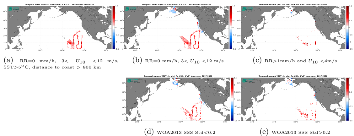
Figure 14: Temporal mean gridded over spatial boxes of size 1^\circ \times 1^\circ of \Delta\text{SSS} (SMOS SSS L4 v2 - Daily (BEC) - Sairdrone) for 5 different subdatasets corresponding to:RR=0 mm/h, 3 < U_{10} < 12 m/s, SST >5^\circ\text{C} , distance to coast > 800 km (a), RR=0 mm/h, 3 < U_{10} < 12 m/s (b), RR >1 mm/h and U_{10} < 4 m/s (c), WOA2013 SSS Std <0.2 (d), WOA2013 SSS Std >0.2 (e).
