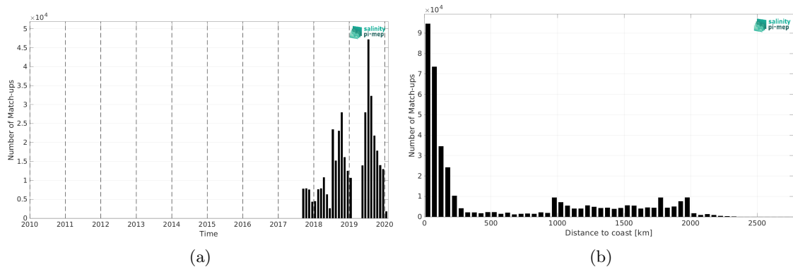
Figure 2: Number of match-ups between Saildrone and SMOS SSS L4 v2 - Daily (BEC) SSS as a function of time (a) and as function of the distance to coast (b) over the North Pacific Ocean Pi-MEP region and for the full satellite product period.
