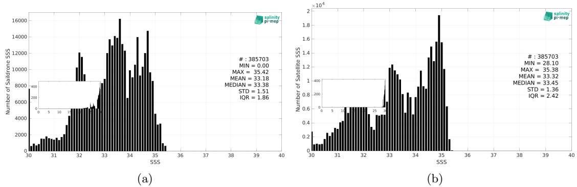
Figure 3: Histograms of SSS from Saildrone (a) and SMOS SSS L4 v2 - Daily (BEC) (b) considering all match-up pairs per bins of 0.1 over the North Pacific Ocean Pi-MEP region and for the full satellite product period.
