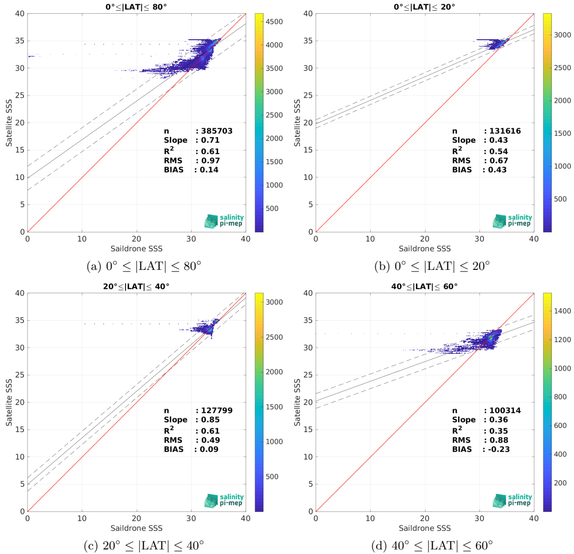
Figure 10: Contour maps of the concentration of SMOS SSS L4 v2 - Daily (BEC) SSS (y-axis) versus Sairdrone SSS (x-axis) at match-up pairs for different latitude bands. For each plot, the red line shows x=y . The black thin and dashed lines indicate a linear fit through the data cloud and the \pm 95\% confidence levels, respectively. The number match-up pairs n , the slope and R^2 coefficient of the linear fit, the root mean square (RMS) and the mean bias between satellite and in situ data are indicated for each latitude band in each plots.
