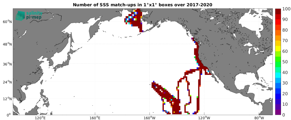
Figure 5: Number of SSS match-ups between Saildrone SSS and the SMOS SSS L4 v2 - Daily (BEC) SSS product for the North Pacific Ocean Pi-MEP region over 1^\circ \times 1^\circ boxes and for the full satellite product period.
