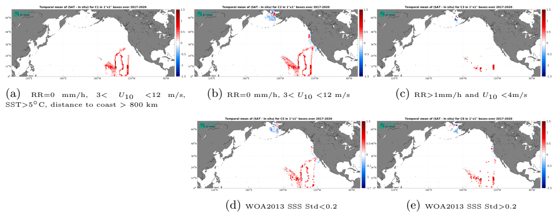
Figure 14: Temporal mean gridded over spatial boxes of size 1^\circ \times 1^\circ of \Delta SSS (SMOS SSS L4 v2 - Daily (BEC) - Sairdrone) for 5 different subdatasets corresponding to:RR=0 mm/h, 3 < U_{10} < 12 m/s, SST >5^\circ\text{C} , distance to coast > 800 km (a), RR=0 mm/h, 3 < U_{10} < 12 m/s (b), RR >1 mm/h and U_{10} < 4 m/s (c), WOA2013 SSS Std <0.2 (d), WOA2013 SSS Std >0.2 (e).
