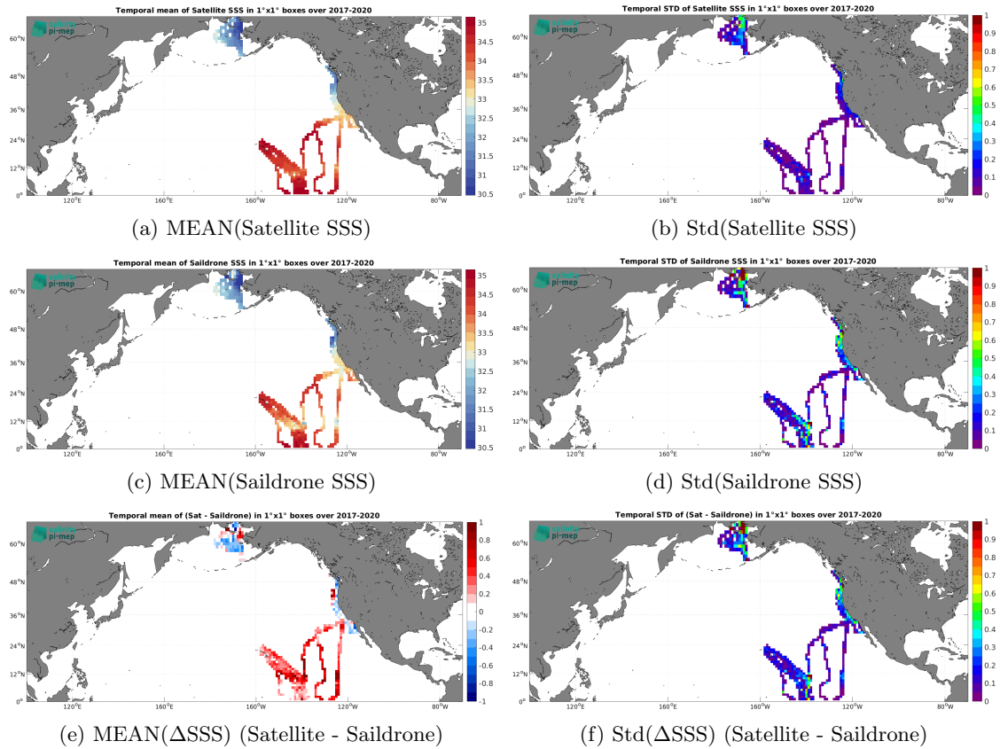
Figure 7: Temporal mean (left) and Std (right) of SSS from SMOS SSS L4 v2 - Daily (BEC) (top), Saildrone (middle), and of \Delta SSS (Satellite - Saildrone). Only match-up pairs are used to generate these maps.
