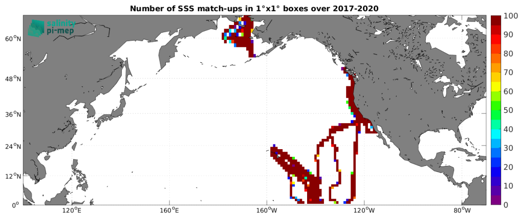
Figure 4: Number of SSS match-ups between Saildrone SSS and the SMOS SSS L4 v2 - Daily (BEC) SSS product for the North Pacific Ocean Pi-MEP region over 1^\circ \times 1^\circ boxes and for the full satellite product period.
