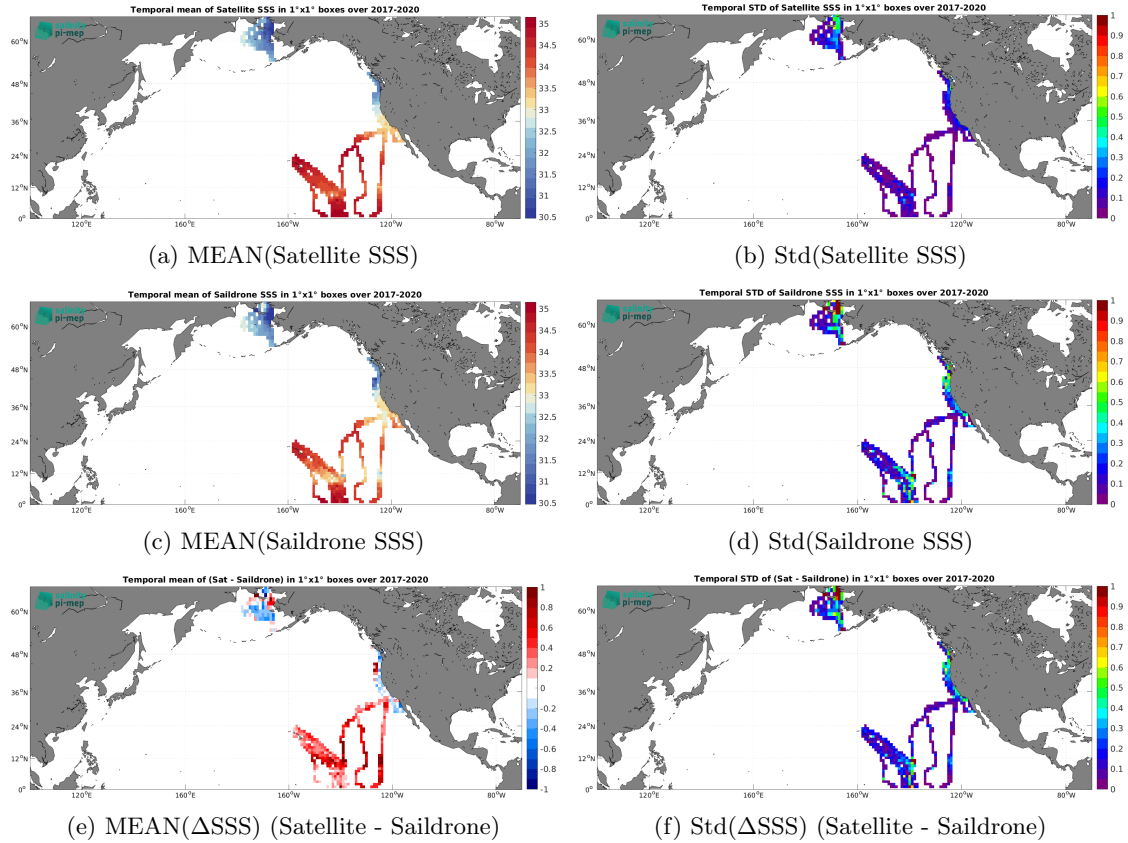
Figure 6: Temporal mean (left) and Std (right) of SSS from SMOS SSS L4 v2 - Daily (BEC) (top), Saildrone (middle), and of \Delta SSS (Satellite - Saildrone). Only match-up pairs are used to generate these maps.
