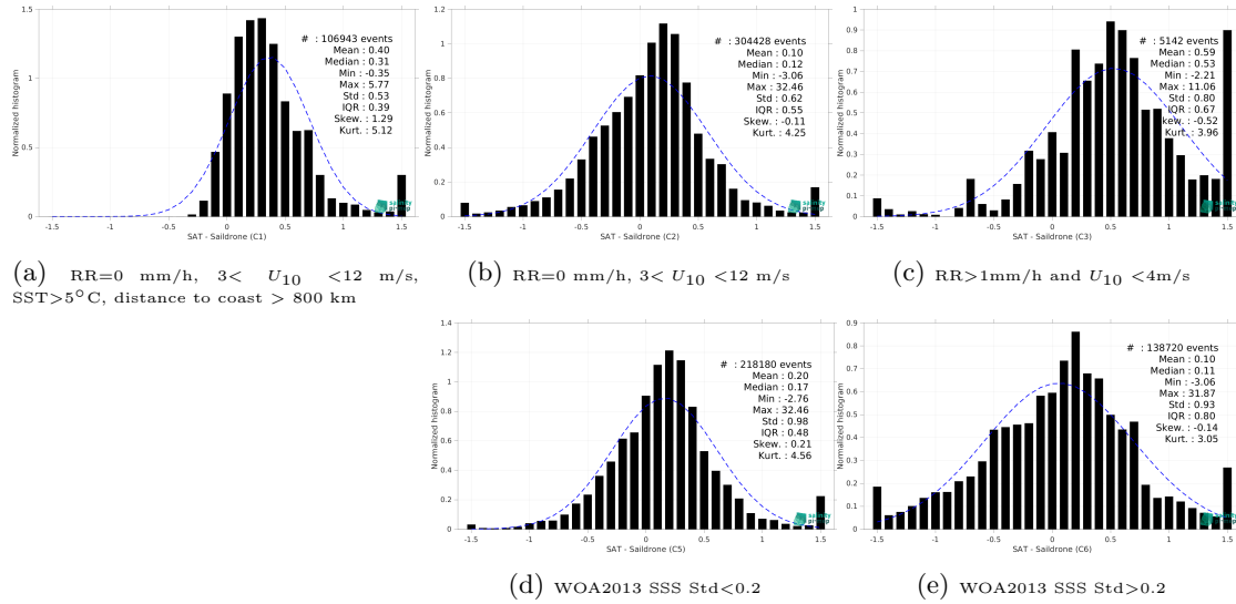
Figure 13: Normalized histogram of \Delta\text{SSS} (SMOS SSS L4 v2 - Daily (BEC) - Saildrone) for 5 different subdatasets corresponding to: RR=0 mm/h, 3 < U_{10} < 12 m/s, SST>5°C, distance to coast > 800 km (a), RR=0 mm/h, 3 < U_{10} < 12 m/s (b), RR>1mm/h and U_{10} < 4 m/s (c), WOA2013 SSS Std<0.2 (d), WOA2013 SSS Std>0.2 (e).
