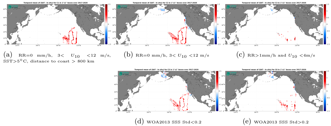
Figure 12: Temporal mean gridded over spatial boxes of size 1^\circ \times 1^\circ of \Delta SSS (SMOS SSS L4 v2 - Daily (BEC) - Sairdrone) for 5 different subdatasets corresponding to:RR=0 mm/h, 3 < U_{10} < 12 m/s, SST >5^\circ C, distance to coast > 800 km (a), RR=0 mm/h, 3 < U_{10} < 12 m/s (b), RR >1 mm/h and U_{10} < 4 m/s (c), WOA2013 SSS Std <0.2 (d), WOA2013 SSS Std >0.2 (e).
