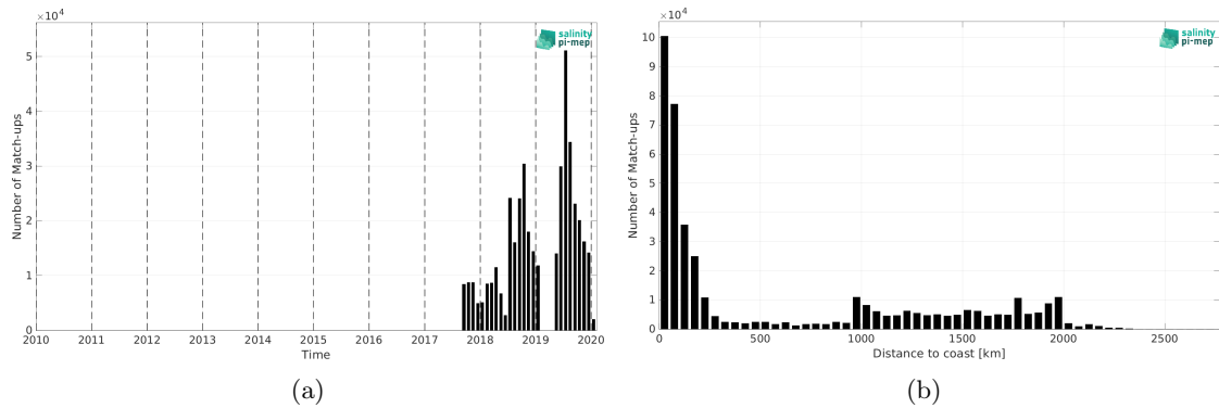
Figure 1: Number of match-ups between Saildrone and SMOS SSS L4 v2 - Daily (BEC) SSS as a function of time (a) and as function of the distance to coast (b) over the North Pacific Ocean Pi-MEP region and for the full satellite product period.
