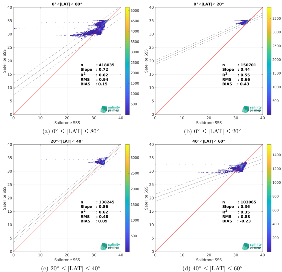
Figure 9: Contour maps of the concentration of SMOS SSS L4 v2 - Daily (BEC) SSS (y-axis) versus Sairdrone SSS (x-axis) at match-up pairs for different latitude bands. For each plot, the red line shows x=y . The black thin and dashed lines indicate a linear fit through the data cloud and the \pm 95\% confidence levels, respectively. The number match-up pairs n , the slope and R^2 coefficient of the linear fit, the root mean square (RMS) and the mean bias between satellite and in situ data are indicated for each latitude band in each plots.
