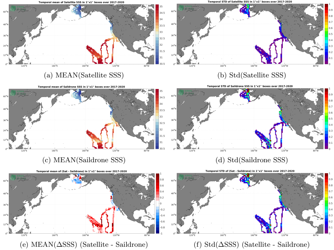
Figure 6: Temporal mean (left) and Std (right) of SSS from SMOS SSS L4 v2 - Daily (BEC) (top), Sairdrone (middle), and of \Delta\text{SSS} (Satellite - Sairdrone). Only match-up pairs are used to generate these maps.
