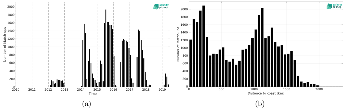
Figure 1: Number of match-ups between Marine mammals and SMOS SSS L4 v2 - Daily (BEC) SSS as a function of time (a) and as function of the distance to coast (b) over the North Pacific Ocean Pi-MEP region and for the full satellite product period.
