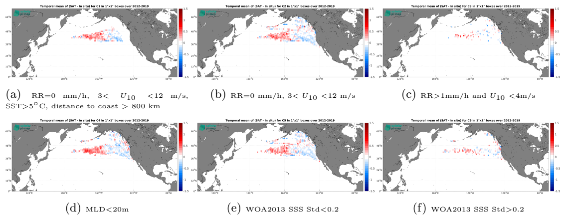
Figure 12: Temporal mean gridded over spatial boxes of size 1^\circ \times 1^\circ of \Delta SSS (SMOS SSS L4 v2 - Daily (BEC) - Marine mammals) for 6 different subdatasets corresponding to:RR=0 mm/h, 3 < U_{10} < 12 m/s, SST >5^\circ\text{C} , distance to coast > 800 km (a), RR=0 mm/h, 3 < U_{10} < 12 m/s (b), RR >1 mm/h and U_{10} < 4 m/s (c),MLD <20 m (d),WOA2013 SSS Std <0.2 (e),WOA2013 SSS Std >0.2 (f).
