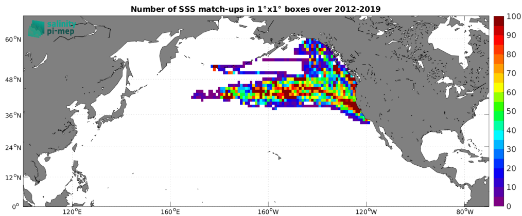
Figure 4: Number of SSS match-ups between Marine mammals SSS and the SMOS SSS L4 v2 - Daily (BEC) SSS product for the North Pacific Ocean Pi-MEP region over 1^\circ \times 1^\circ boxes and for the full satellite product period.
