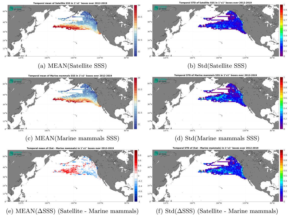
Figure 6: Temporal mean (left) and Std (right) of SSS from SMOS SSS L4 v2 - Daily (BEC) (top), Marine mammals (middle), and of \Delta SSS (Satellite - Marine mammals). Only match-up pairs are used to generate these maps.
