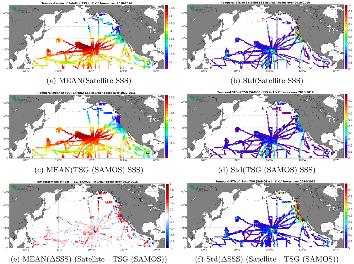
Figure 6: Temporal mean (left) and Std (right) of SSS from SMOS SSS L3 v3 Monthly (ICDC) (top), TSG (SAMOS) (middle), and of \Delta SSS (Satellite - TSG (SAMOS)). Only match-up pairs are used to generate these maps.
