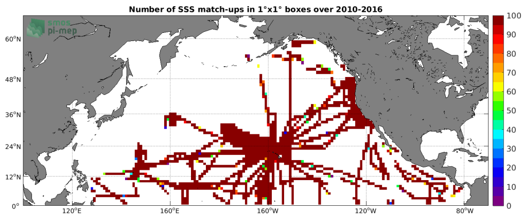
Figure 4: Number of SSS match-ups between TSG (SAMOS) SSS and the SMOS SSS L3 v3 Monthly (ICDC) SSS product for the North Pacific Ocean Pi-MEP region over 1°x1° boxes and for the full satellite product period.
