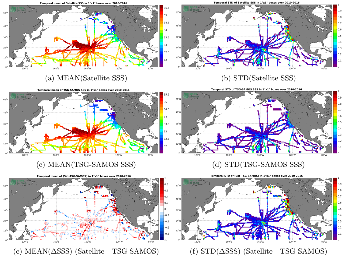
Figure 6: Temporal mean (left) and STD (right) of SSS from SMOS-L3-ICDC-V3-MONTHLY-0.5DEG (top), TSG-SAMOS (middle), and of \Delta SSS (Satellite - TSG-SAMOS). Only match-up pairs are used to generate these maps.
