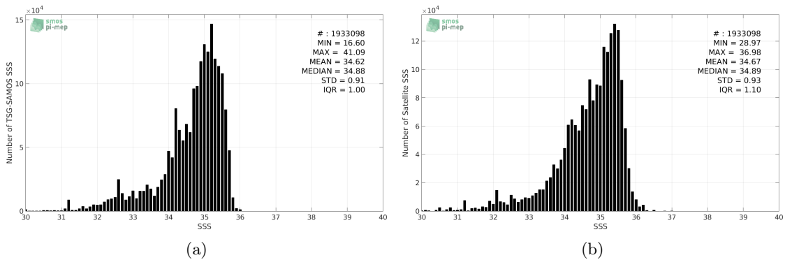
Figure 2: Histograms of SSS from TSG-SAMOS (a) and SMOS-L3-ICDC-V3-MONTHLY-0.5DEG (b) considering all match-up pairs per bins of 0.1 over the North Pacific Ocean Pi-MEP region and for the full satellite product period.
