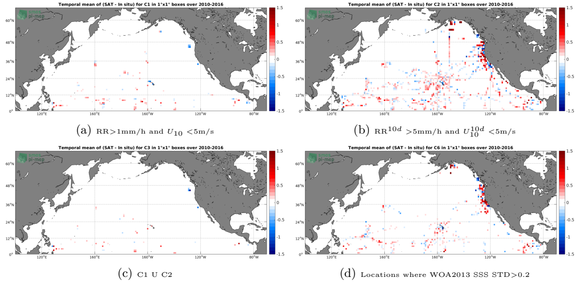
Figure 12: Temporal mean gridded over spatial boxes of size 1^\circ \times 1^\circ of \Delta SSS (SMOS-L3-ICDC-V3-MONTHLY-0.5DEG - TSG-SAMOS) for 4 different subdatasets corresponding to: RR > 1mm/h and U_{10} < 5\text{m/s} (a), RR^{10d} > 5\text{mm/h} and U_{10}^{10d} < 5\text{m/s} (b), C1 U C2 (c), Locations where WOA2013 SSS STD > 0.2 (d).
