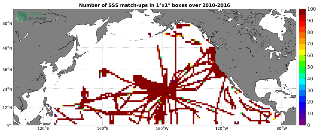
Figure 4: Number of SSS match-ups between TSG-SAMOS SSS and the SMOS-L3-ICDC-V3-MONTHLY-0.5DEG SSS product for the North Pacific Ocean Pi-MEP region over 1^\circ \times 1^\circ boxes and for the full satellite product period.
