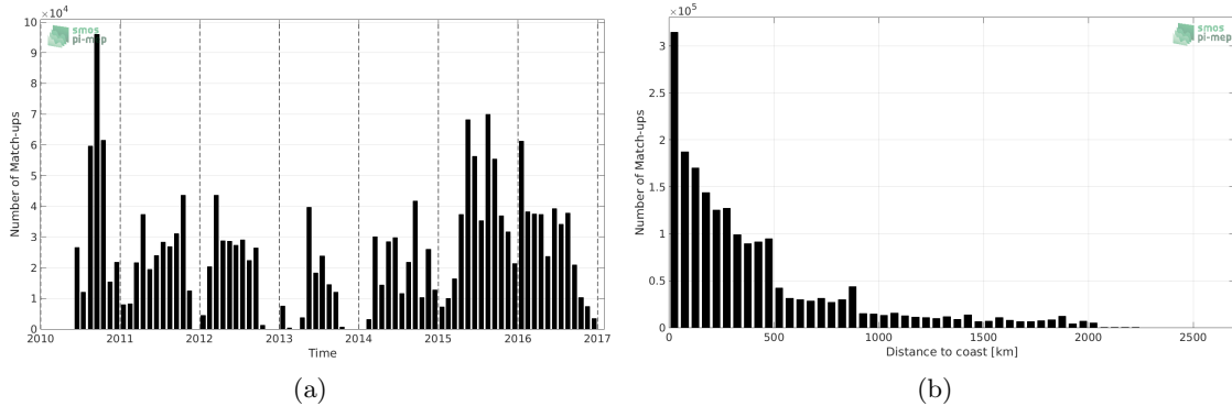
Figure 1: Number of match-ups between TSG-SAMOS and SMOS-L3-ICDC-V3-MONTHLY-0.5DEG SSS as a function of time (a) and as function of the distance to coast (b) over the North Pacific Ocean Pi-MEP region and for the full satellite product period.
