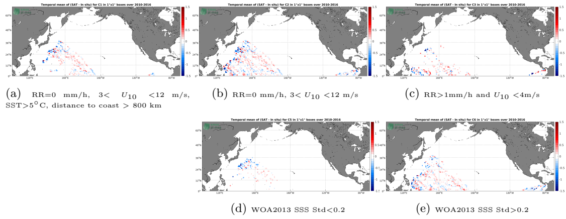
Figure 12: Temporal mean gridded over spatial boxes of size 1^\circ \times 1^\circ of \Delta SSS (SMOS SSS L3 v3 Monthly (ICDC) - TSG (LEGOS-DM)) for 5 different subdatasets corresponding to: RR=0 mm/h, 3 < U_{10} < 12 m/s, SST >5^\circ\text{C} , distance to coast > 800 km (a), RR=0 mm/h, 3 < U_{10} < 12 m/s (b), RR >1 mm/h and U_{10} < 4 m/s (c), WOA2013 SSS Std <0.2 (d), WOA2013 SSS Std >0.2 (e).
