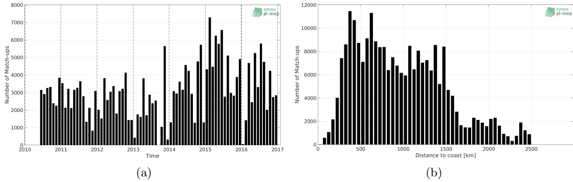
Figure 1: Number of match-ups between TSG (LEGOS-DM) and SMOS SSS L3 v3 Monthly (ICDC) SSS as a function of time (a) and as function of the distance to coast (b) over the North Pacific Ocean Pi-MEP region and for the full satellite product period.
