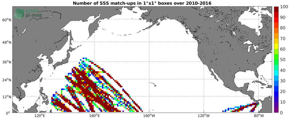
Figure 4: Number of SSS match-ups between TSG (LEGOS-DM) SSS and the SMOS SSS L3 v3 Monthly (ICDC) SSS product for the North Pacific Ocean Pi-MEP region over 1^\circ \times 1^\circ boxes and for the full satellite product period.
