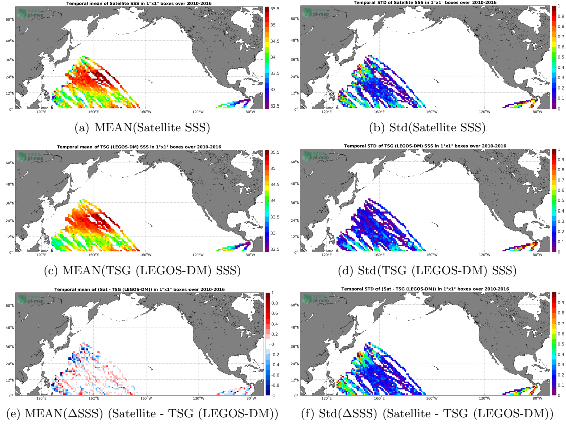
Figure 6: Temporal mean (left) and Std (right) of SSS from SMOS SSS L3 v3 Monthly (ICDC) (top), TSG (LEGOS-DM) (middle), and of \Delta SSS (Satellite - TSG (LEGOS-DM)). Only match-up pairs are used to generate these maps.
