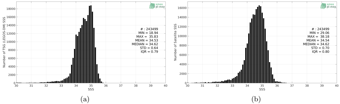
Figure 2: Histograms of SSS from TSG (LEGOS-DM) (a) and SMOS SSS L3 v3 Monthly (ICDC) (b) considering all match-up pairs per bins of 0.1 over the North Pacific Ocean Pi-MEP region and for the full satellite product period.
